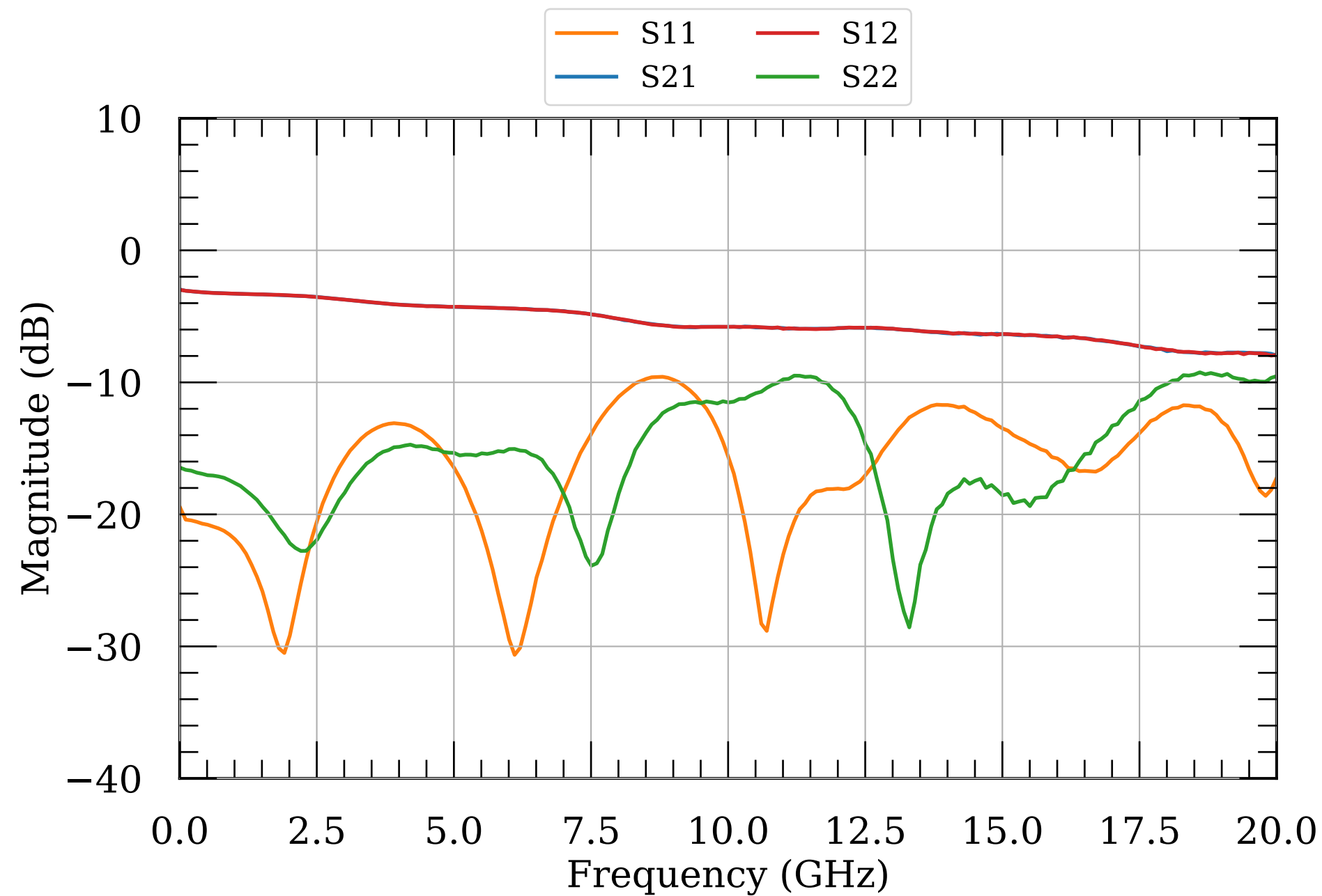
LNA S-params, 1 dBm
