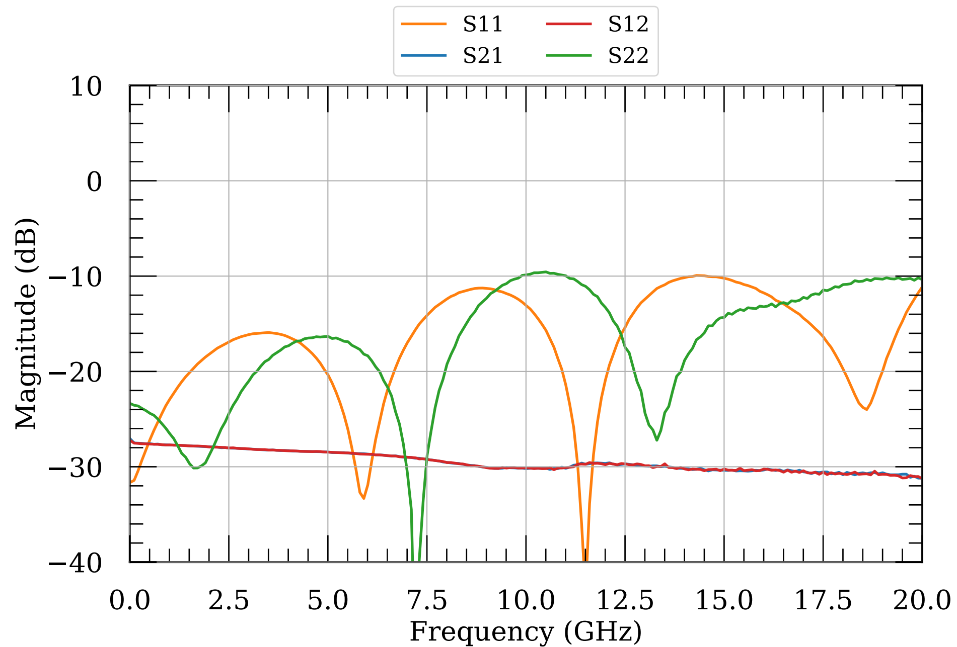
LNA S-params, 25 dBm
