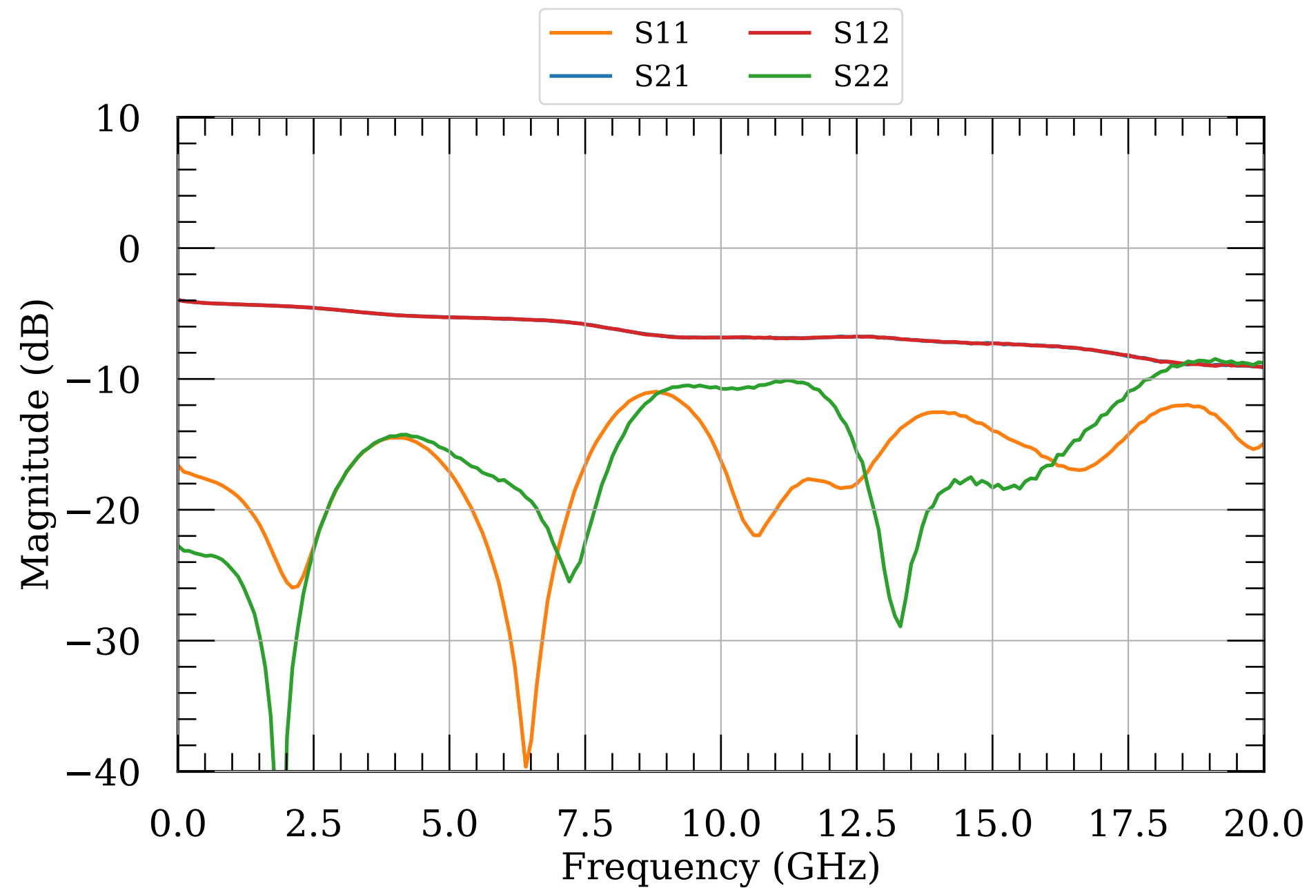
LNA S-params, 2 dBm
