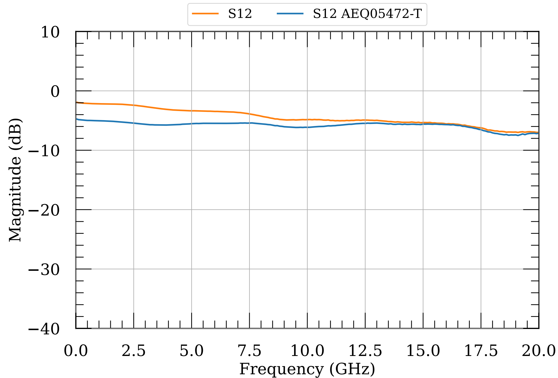
LNA S-params, 0 dBm, S12
