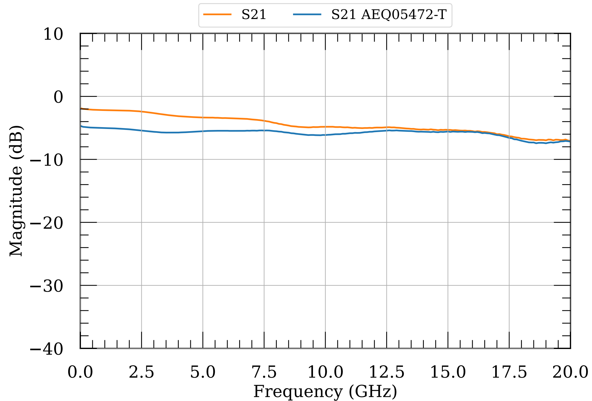
LNA S-params, 0 dBm, S21
