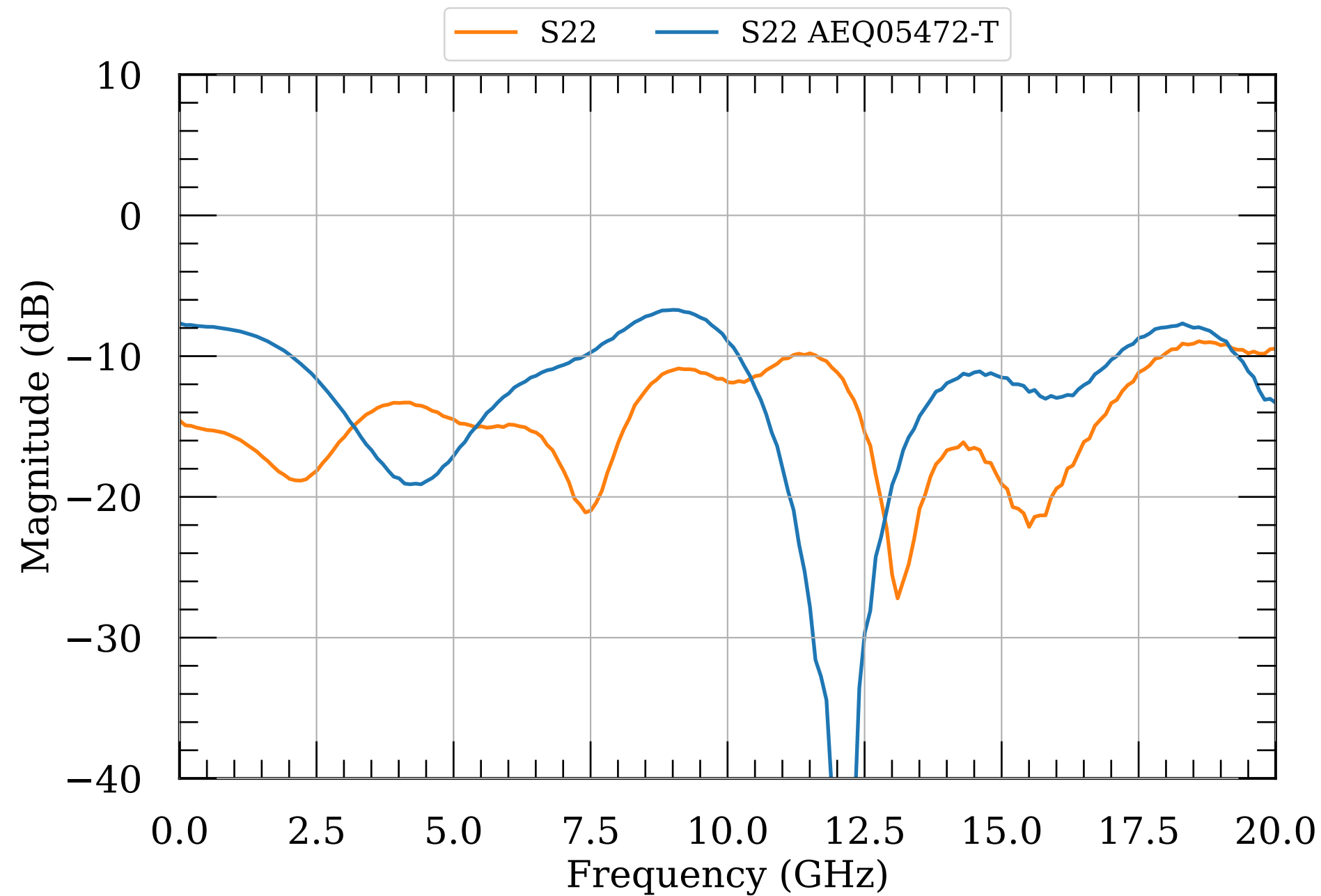
LNA S-params, 0 dBm, S22
