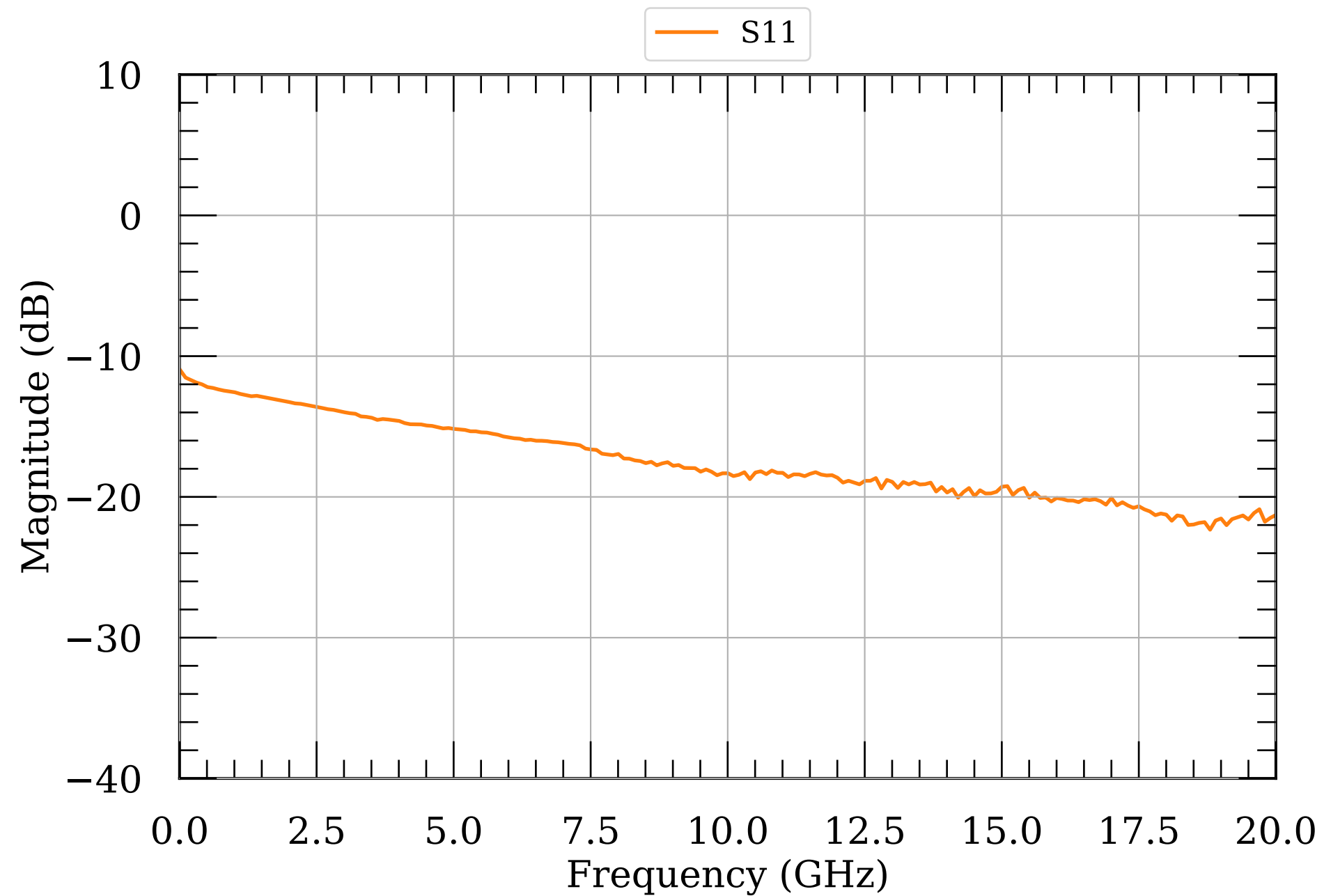
LNA S-params 18.5
