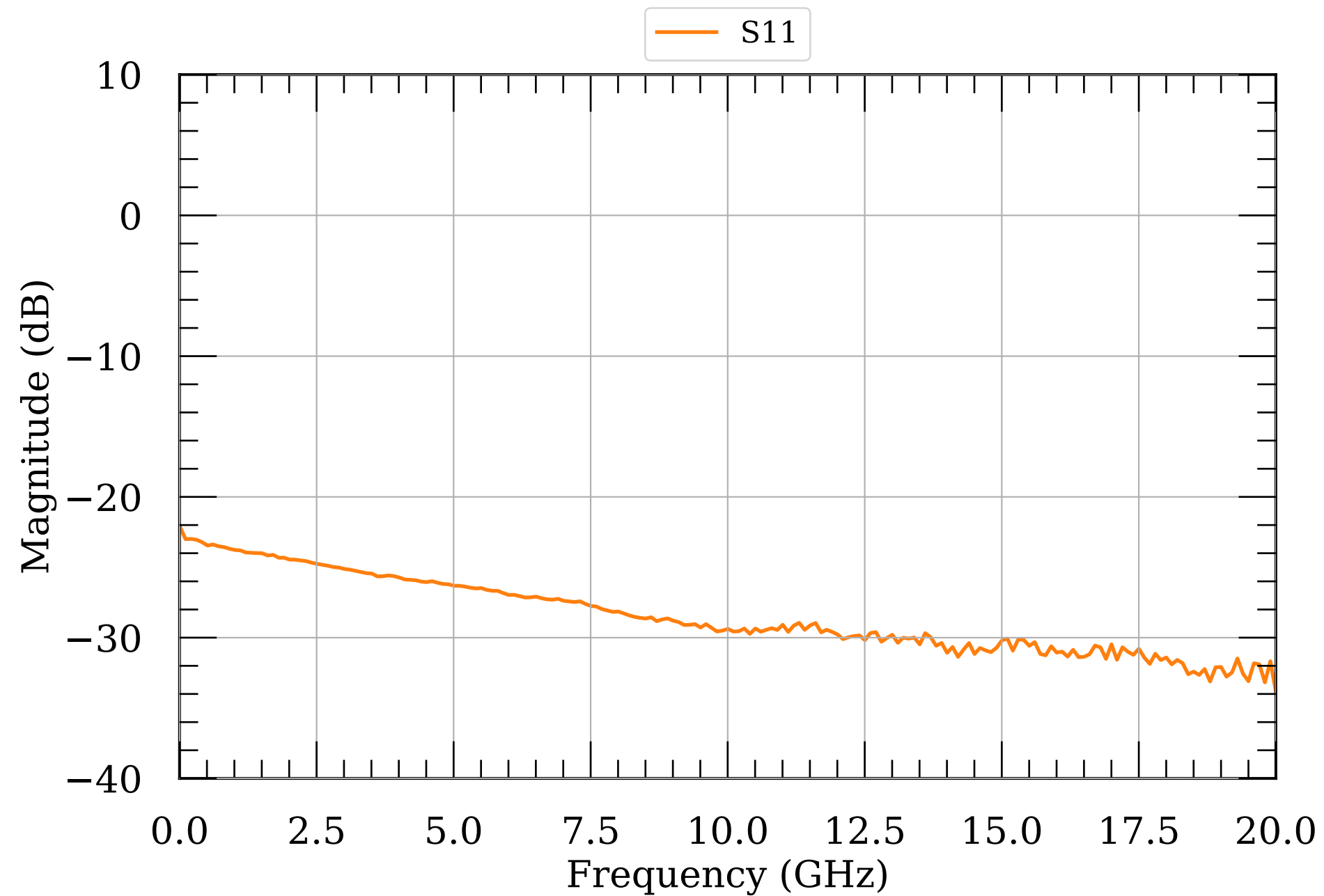
LNA S-params 5.0
