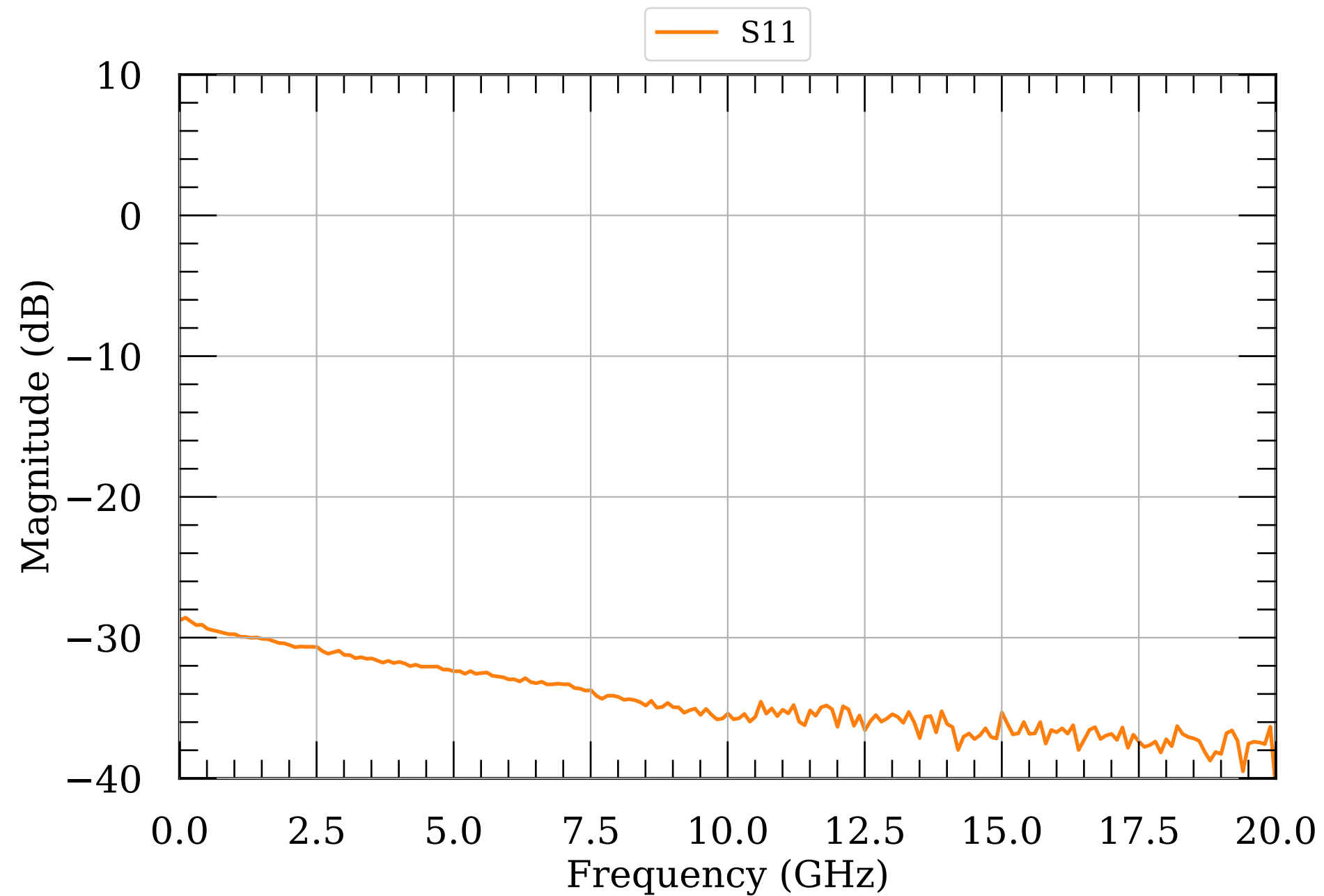
LNA S-params 11.5
