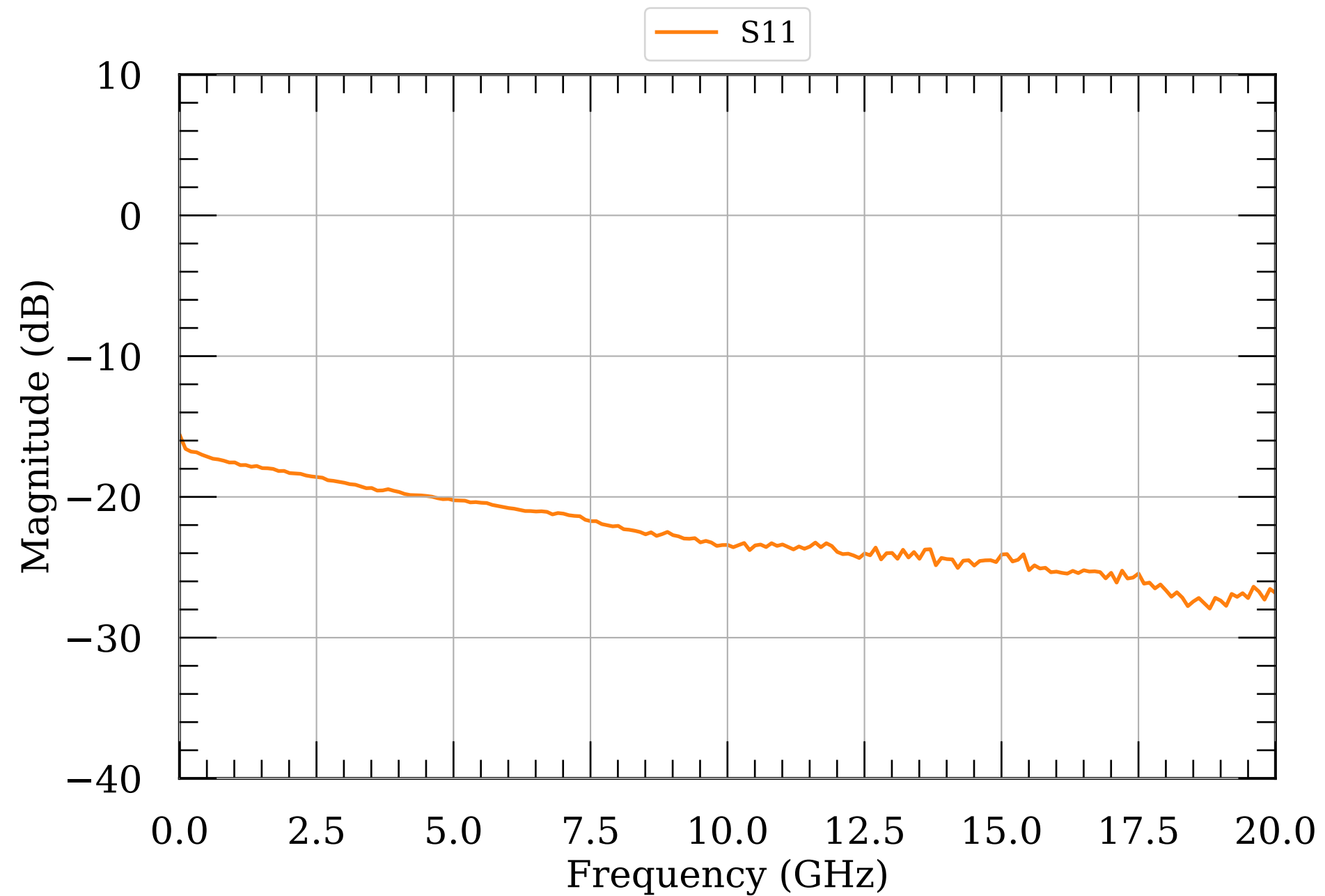
LNA S-params 14.5
