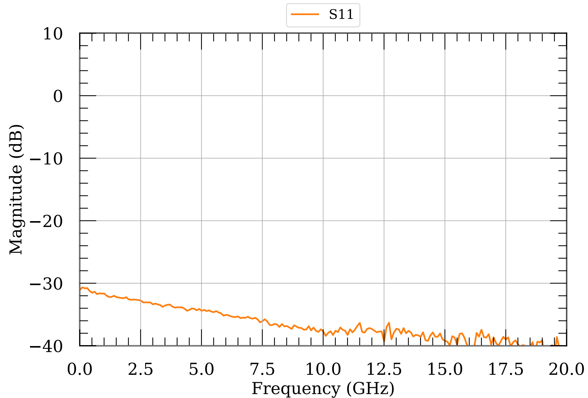
LNA S-params 7.0
