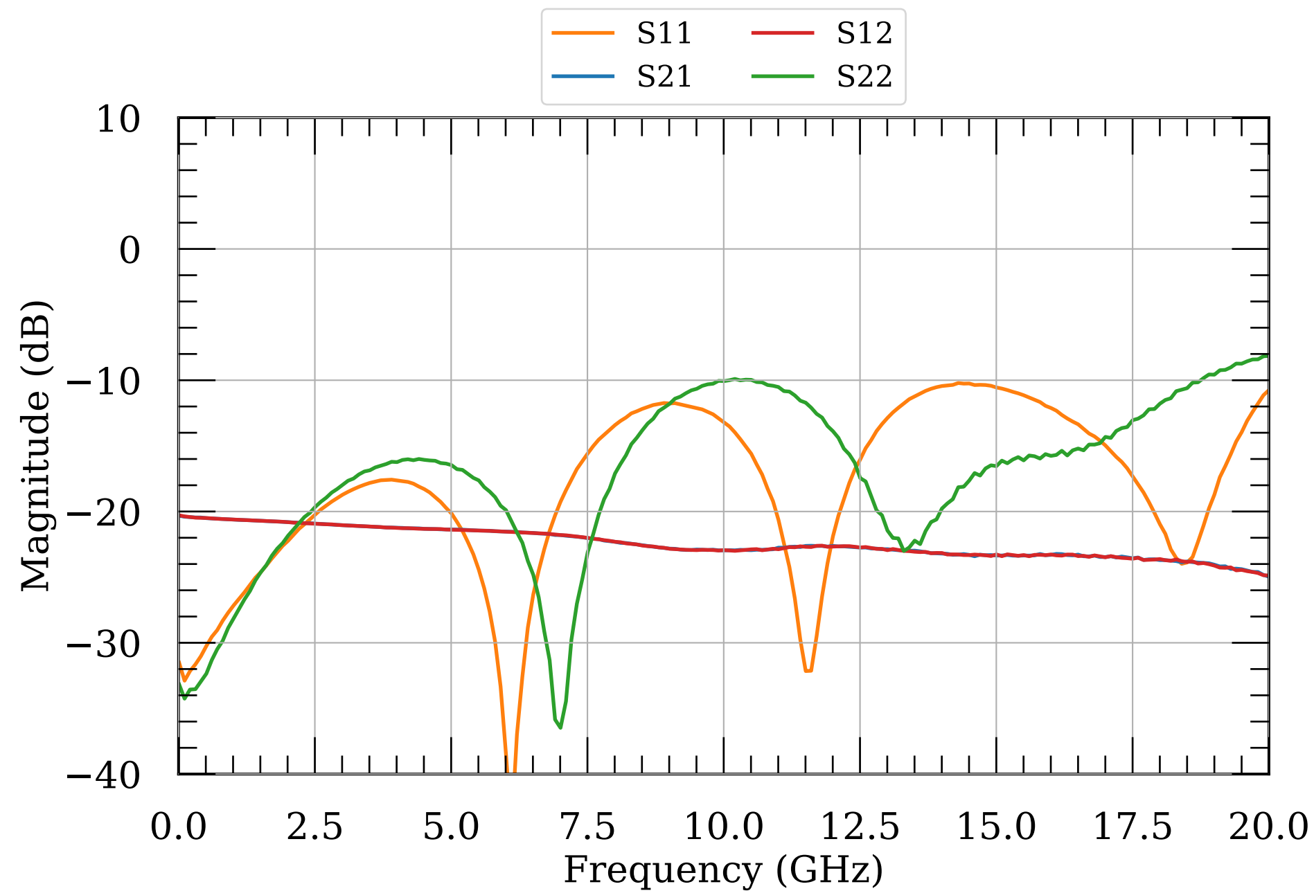
LNA S-params, 18 dBm
