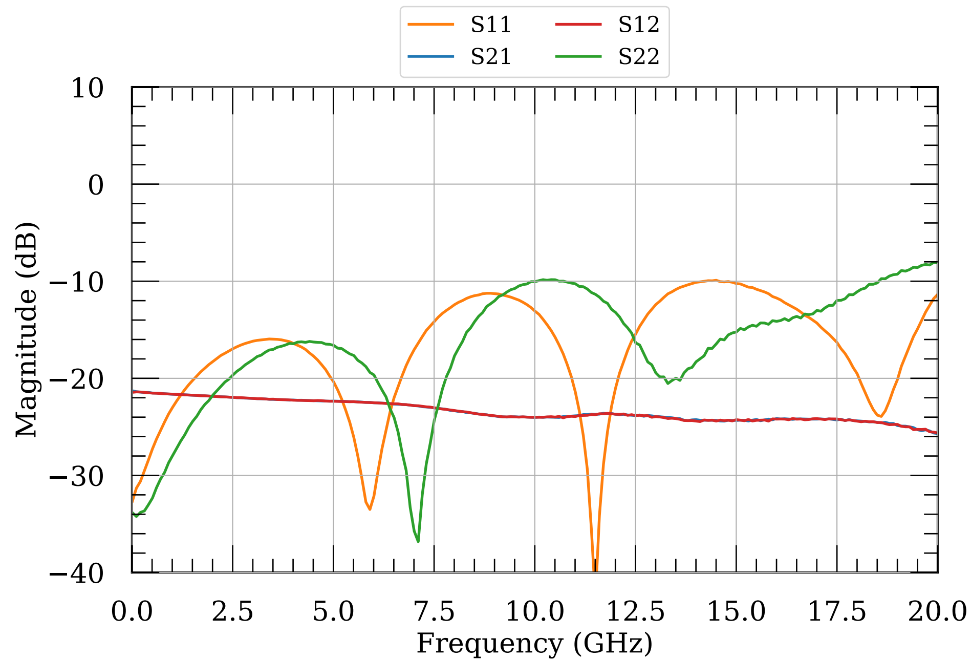
LNA S-params, 19 dBm
