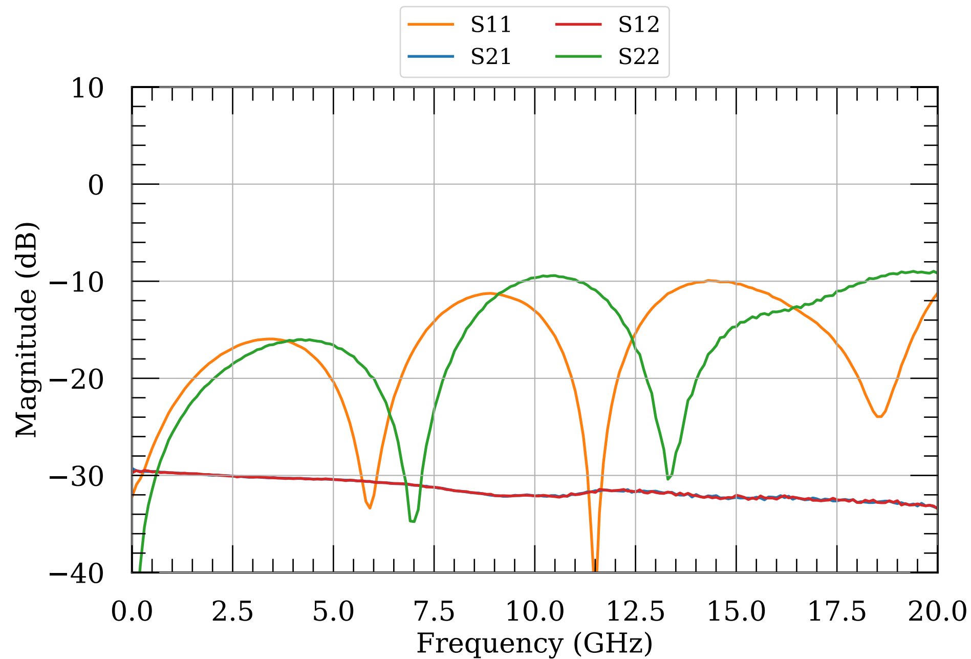
LNA S-params, 27 dBm
