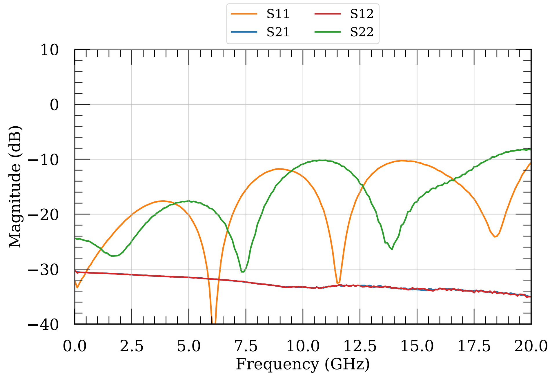
LNA S-params, 28 dBm
