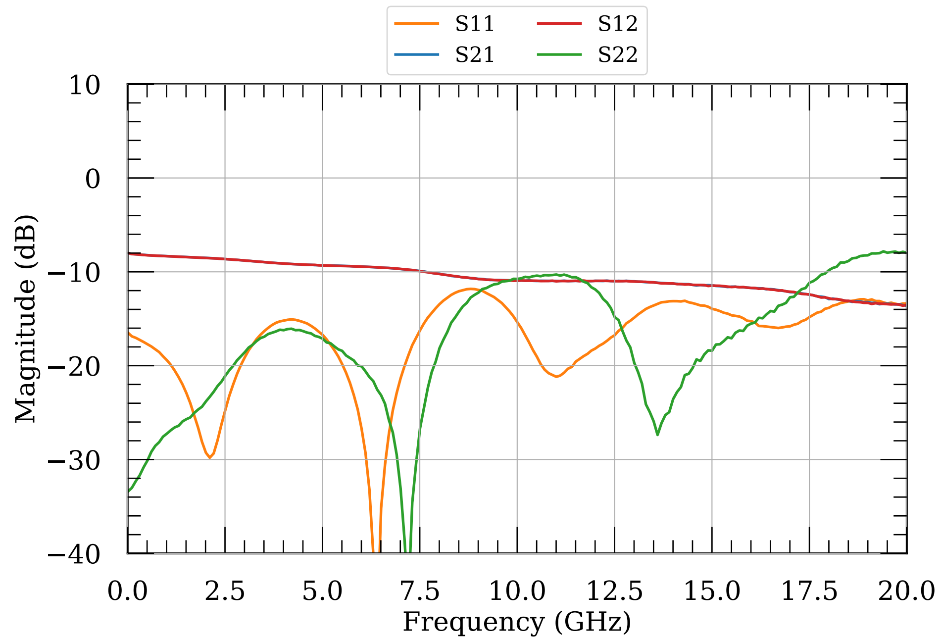
LNA S-params, 6 dBm
