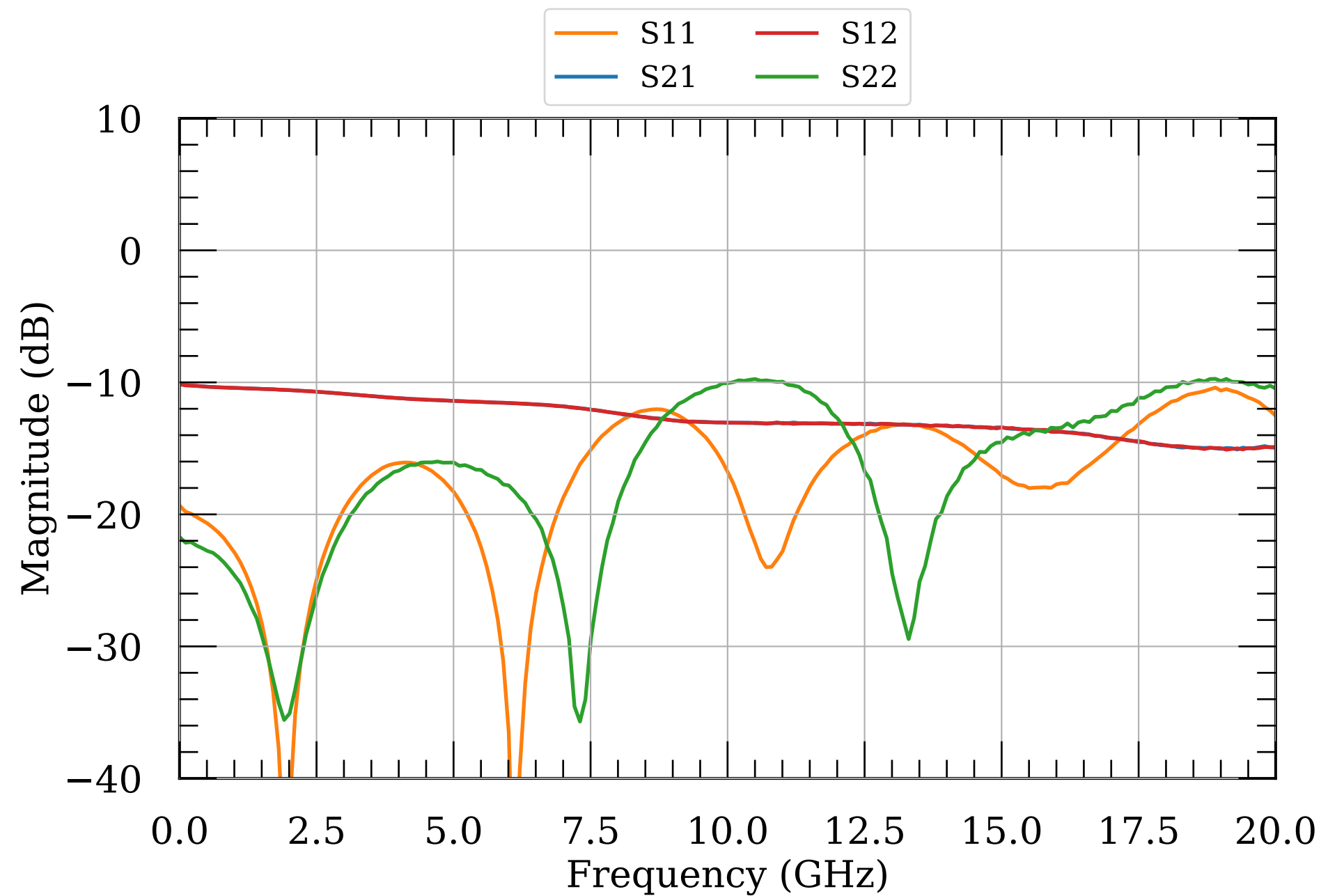
LNA S-params, 8 dBm
