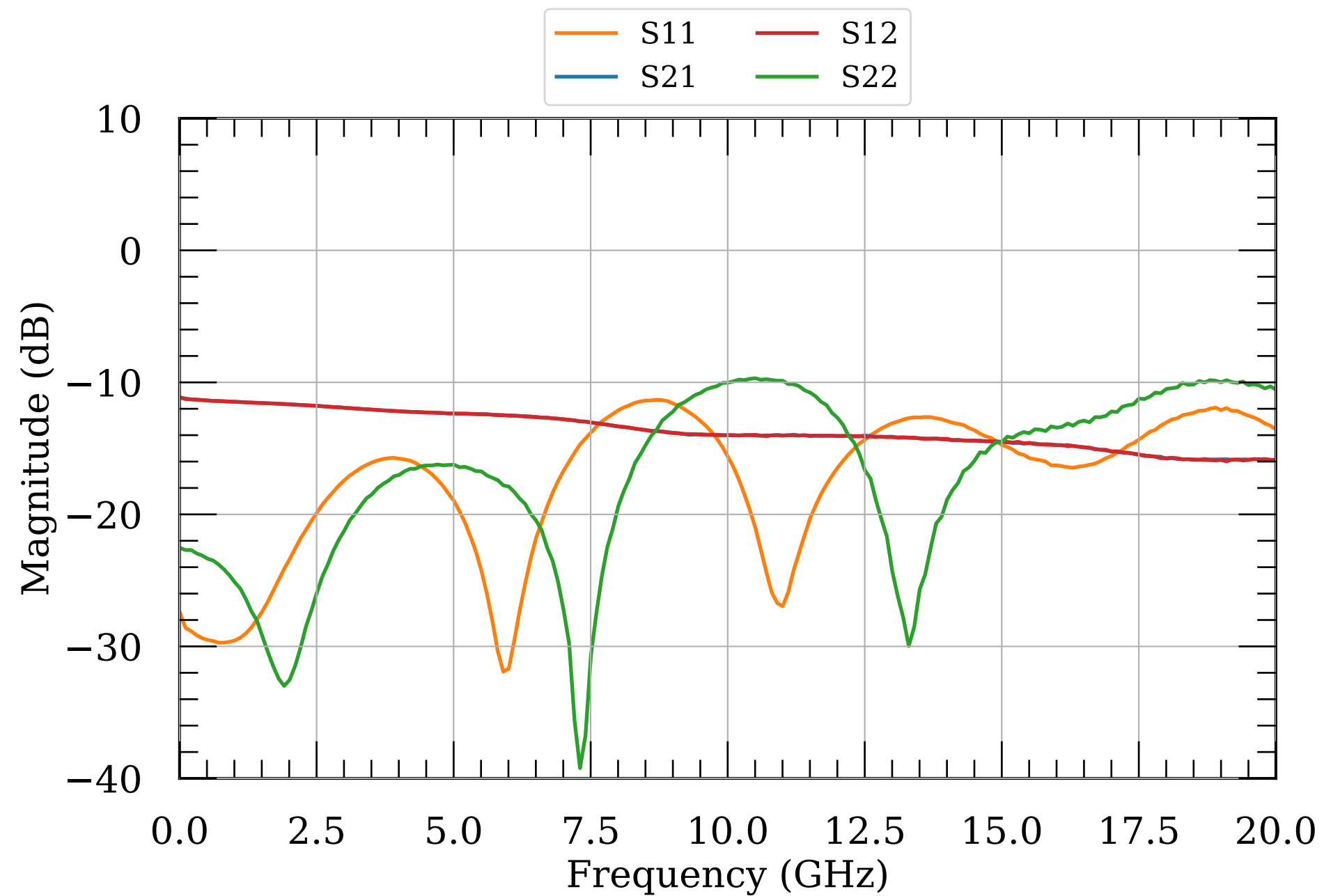
LNA S-params, 9 dBm
