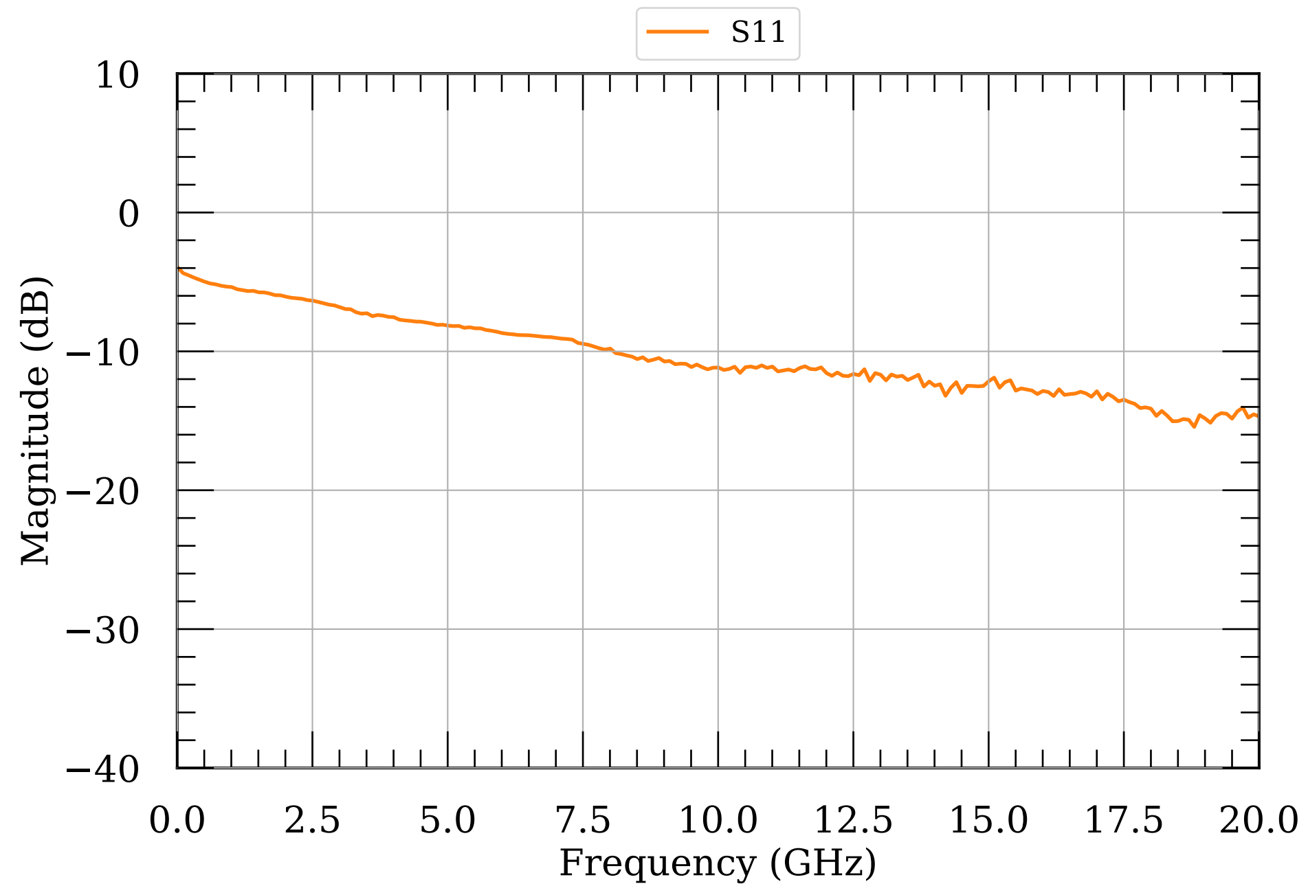
LNA S-params 8.5
