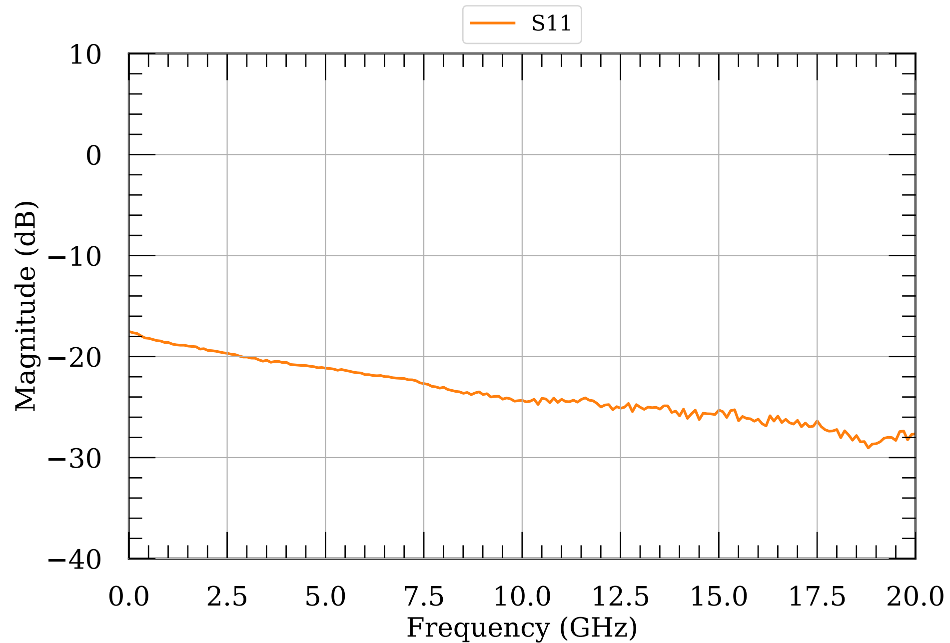
LNA S-params 30.0
