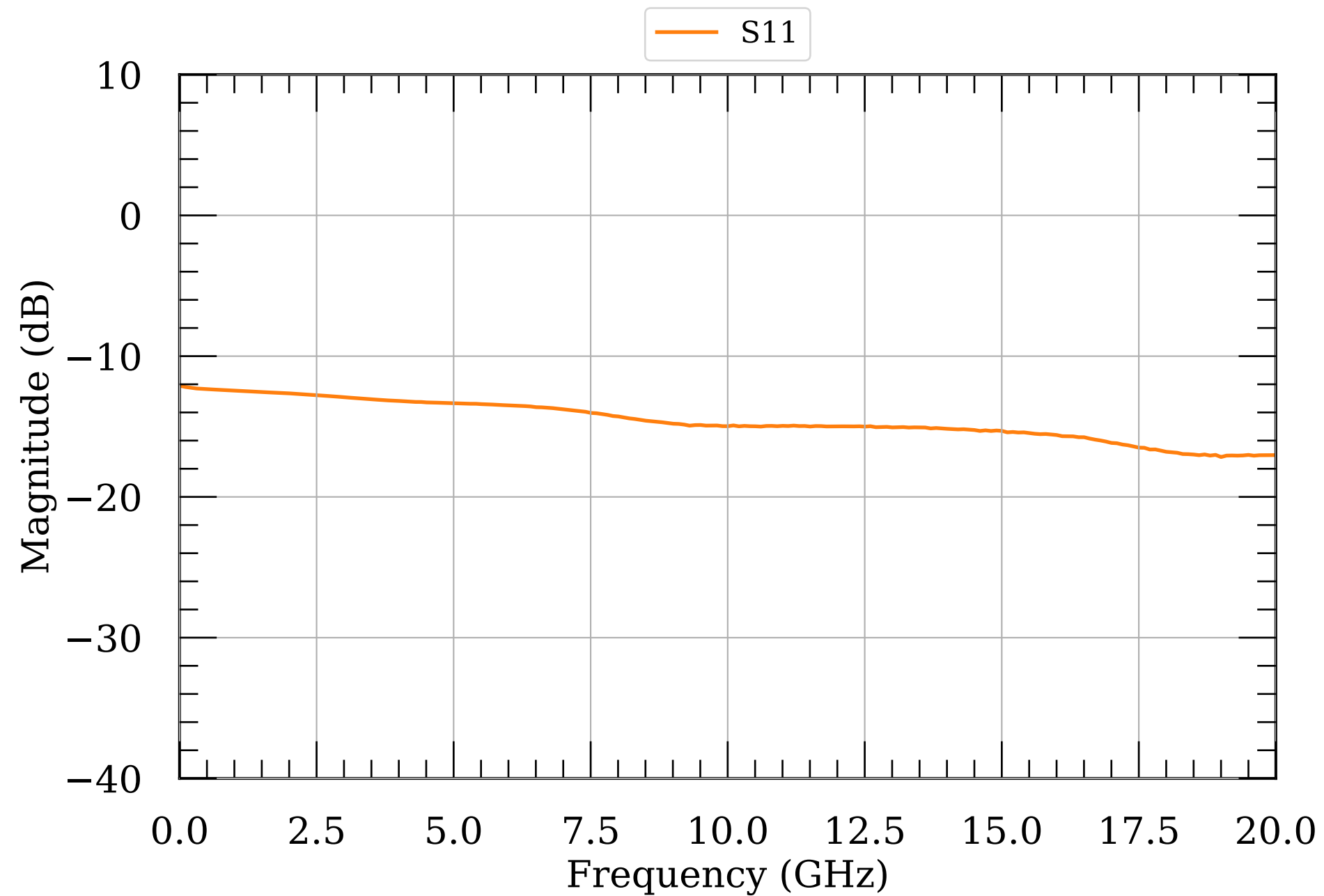
LNA S-params, 10 dBm
