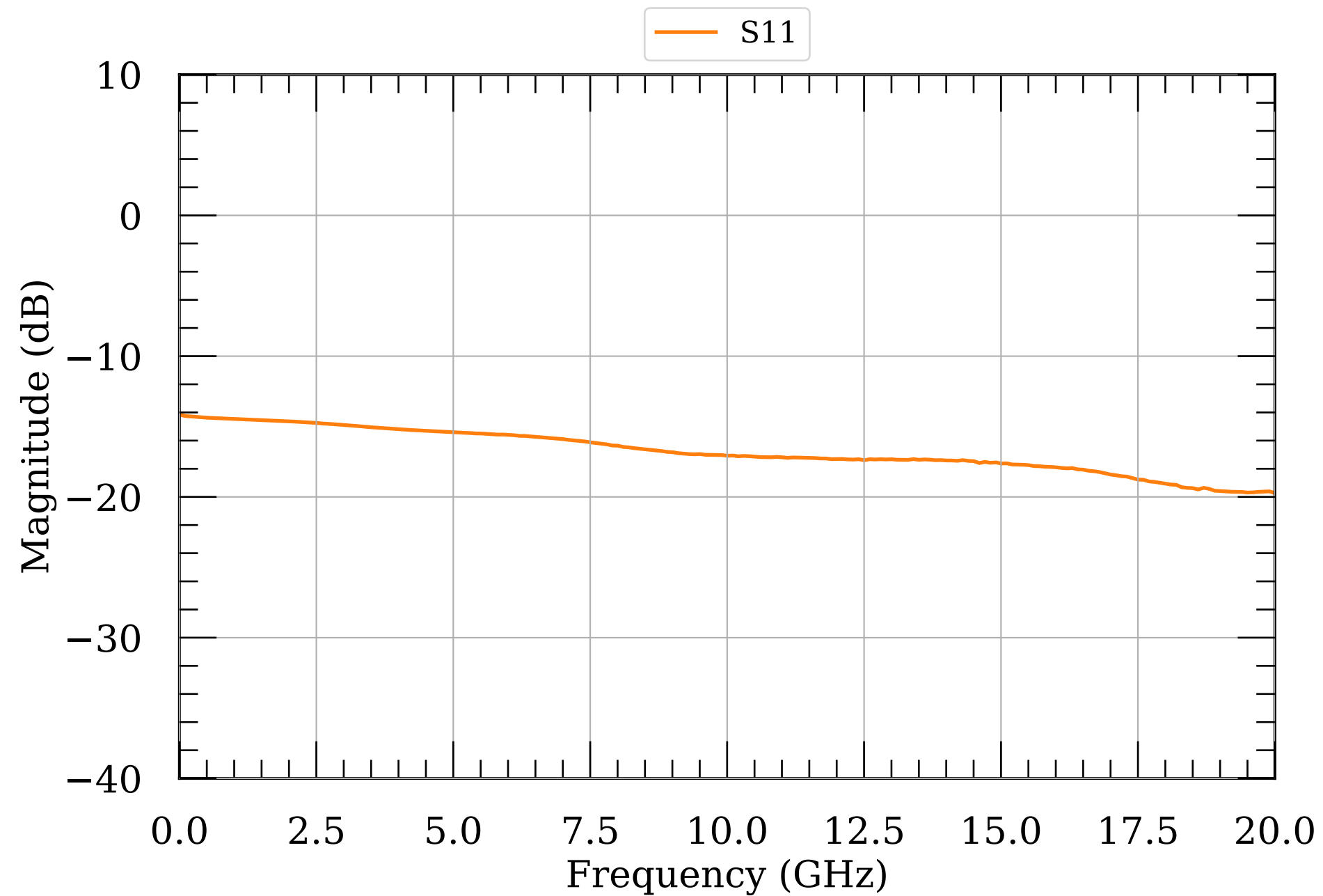
LNA S-params, 12 dBm
