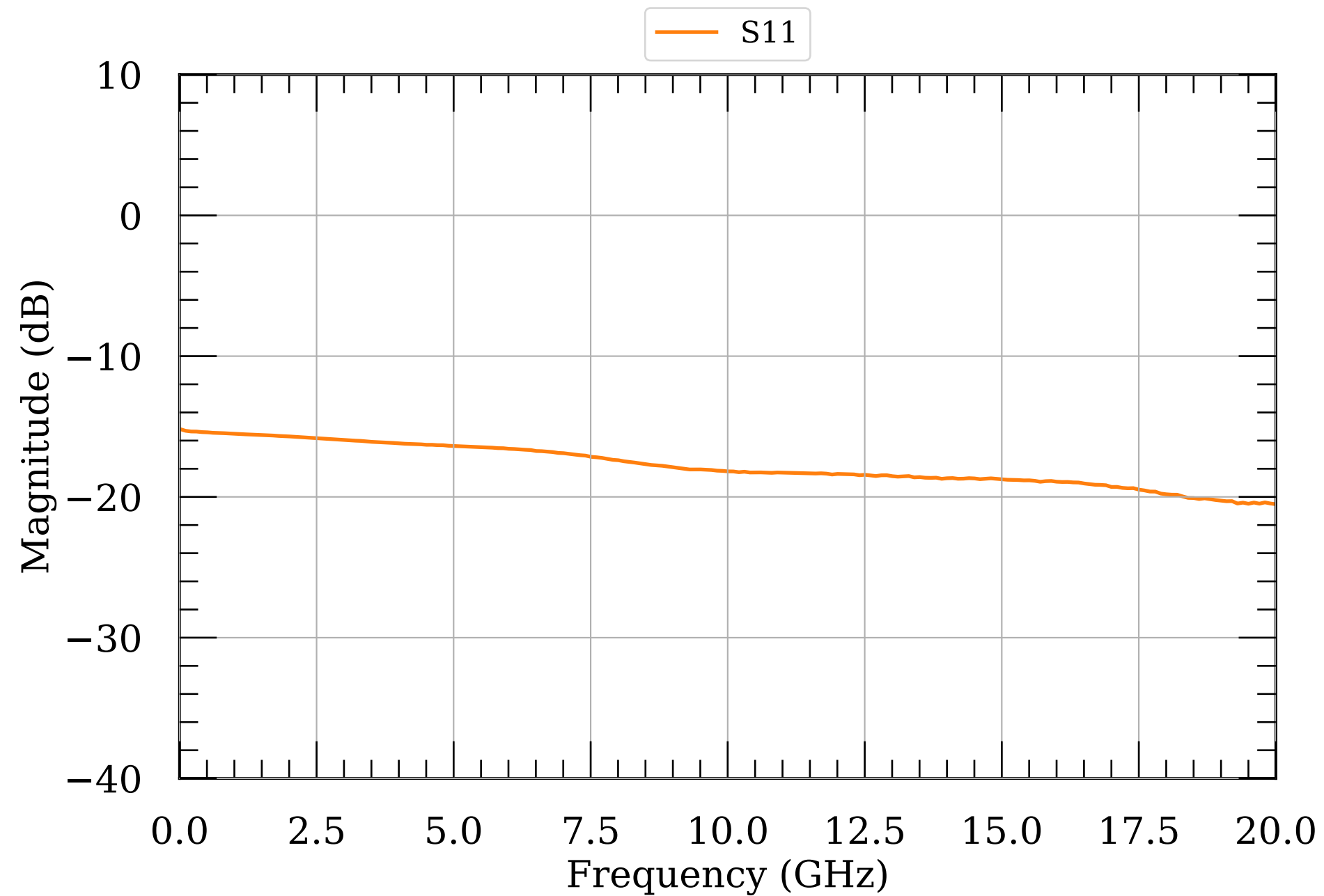
LNA S-params, 13 dBm
