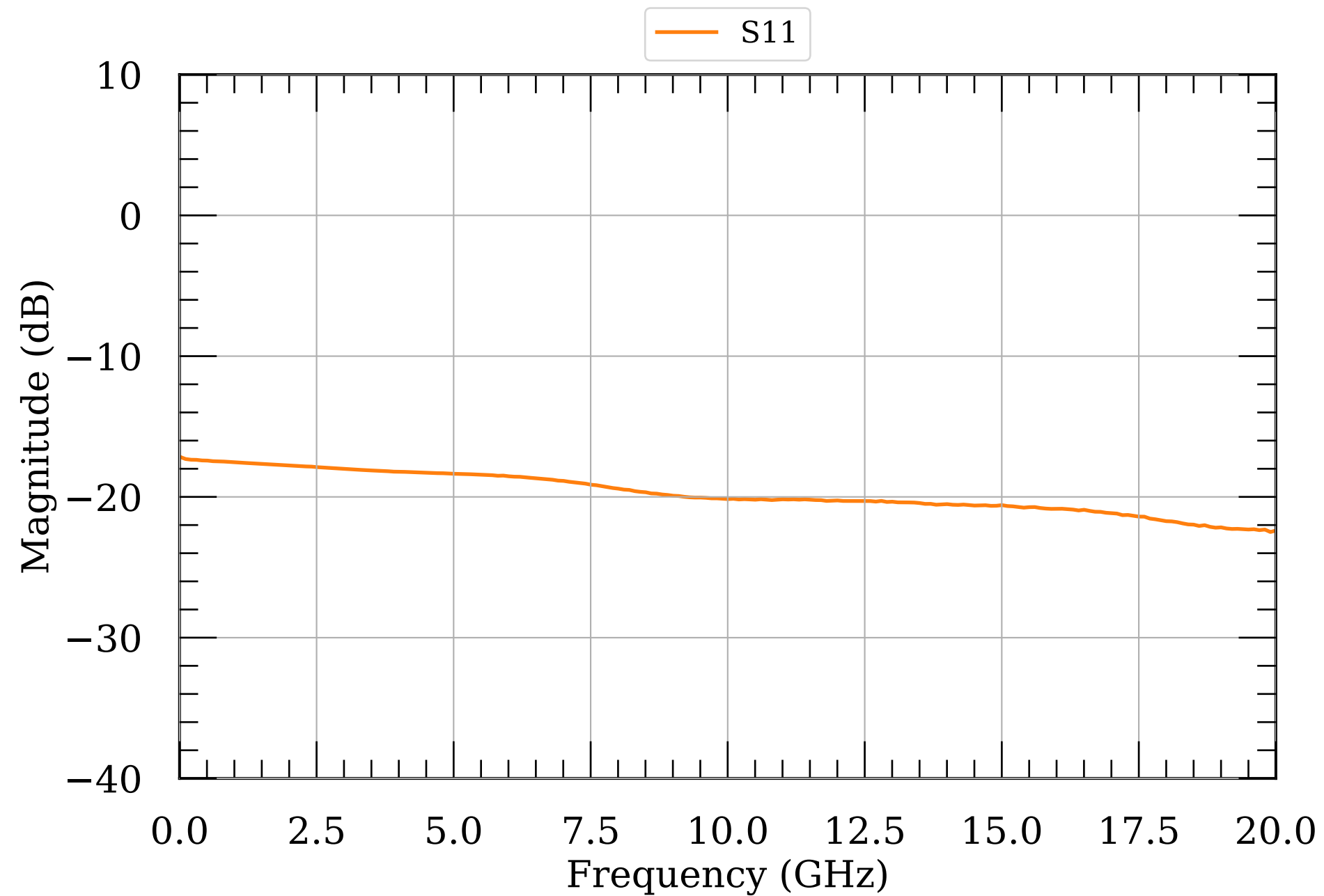
LNA S-params, 15 dBm
