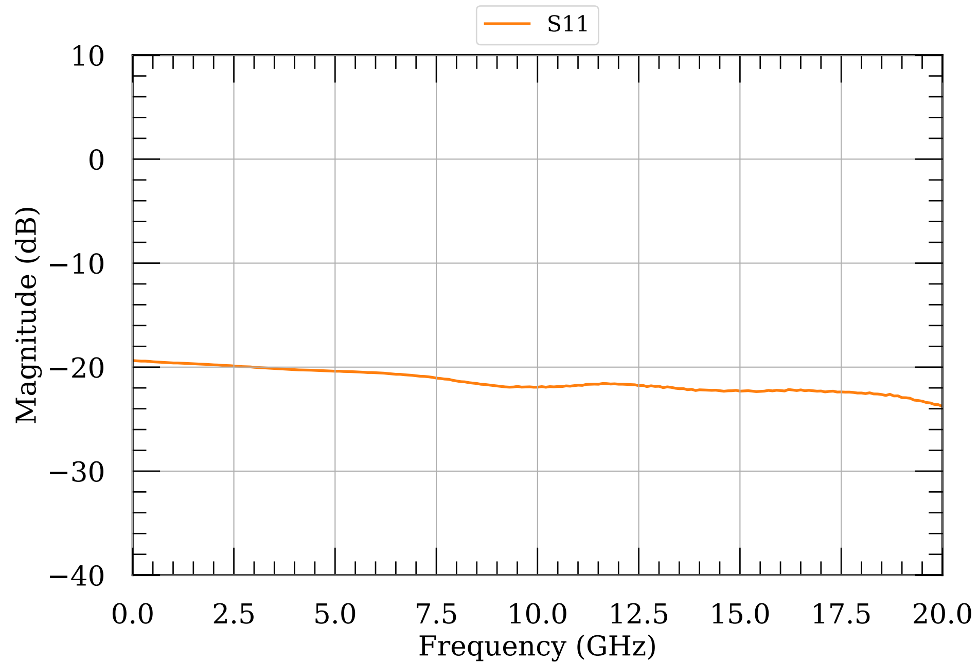
LNA S-params, 17 dBm
