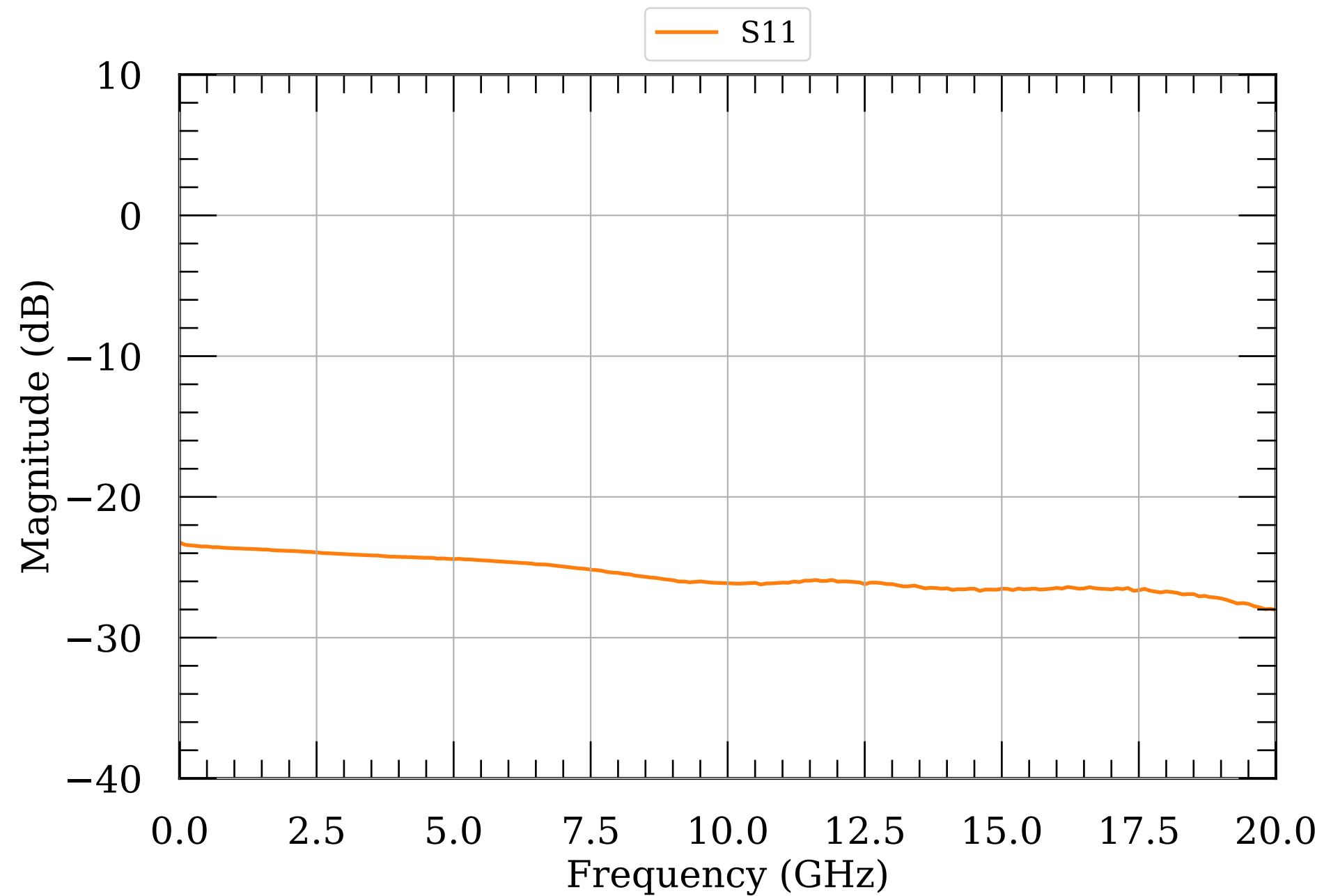
LNA S-params, 21 dBm
