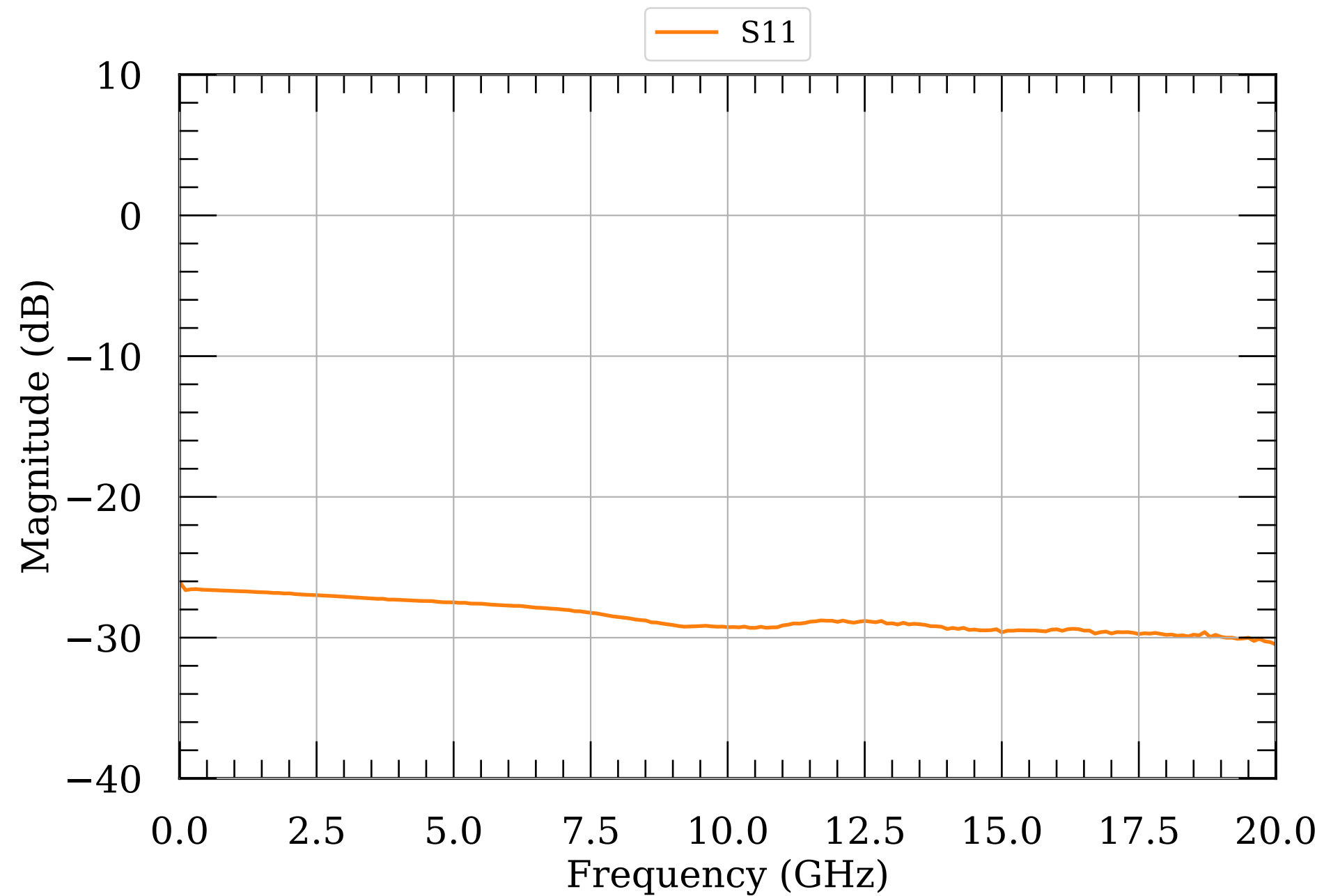
LNA S-params, 24 dBm
