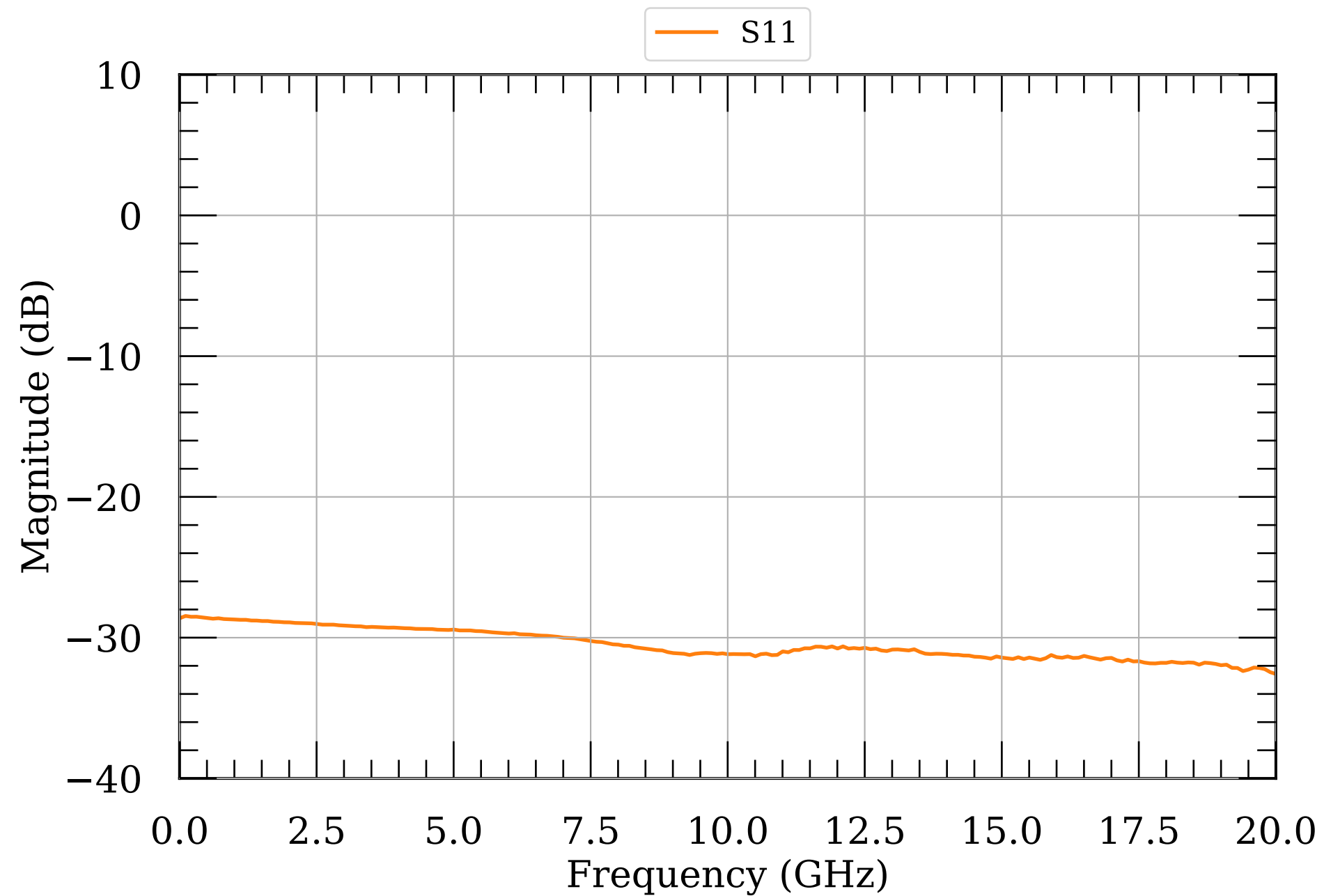
LNA S-params, 26 dBm
