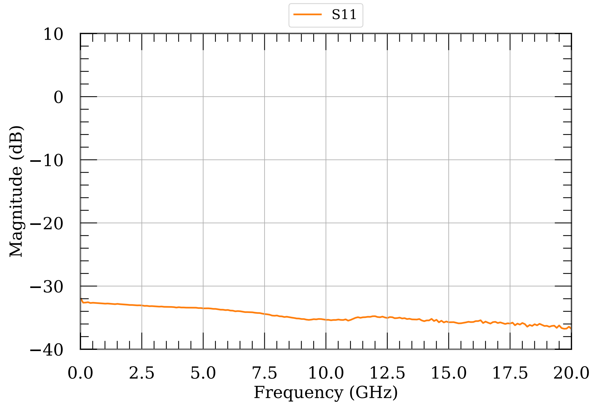
LNA S-params, 30 dBm
