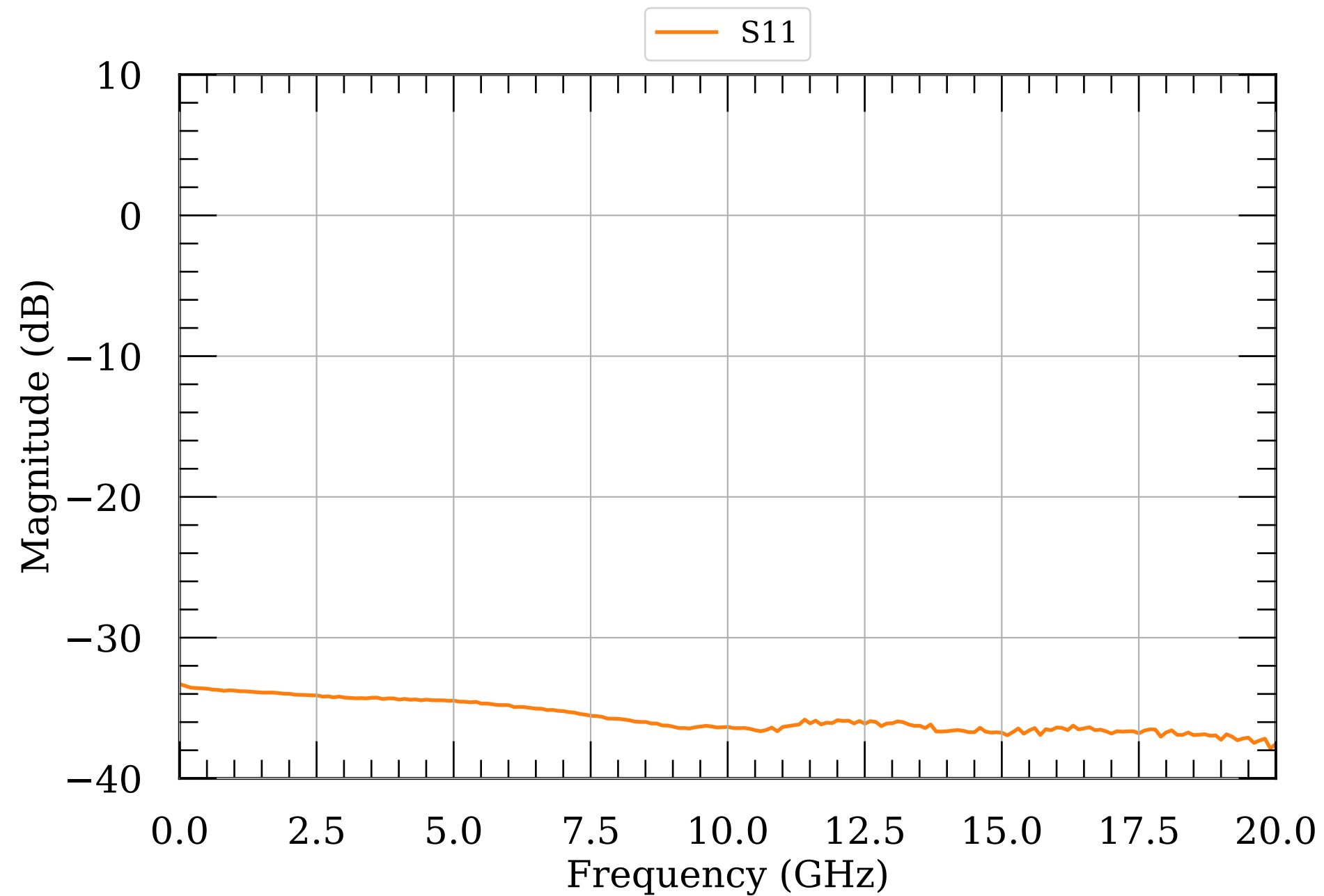
LNA S-params, 31 dBm
