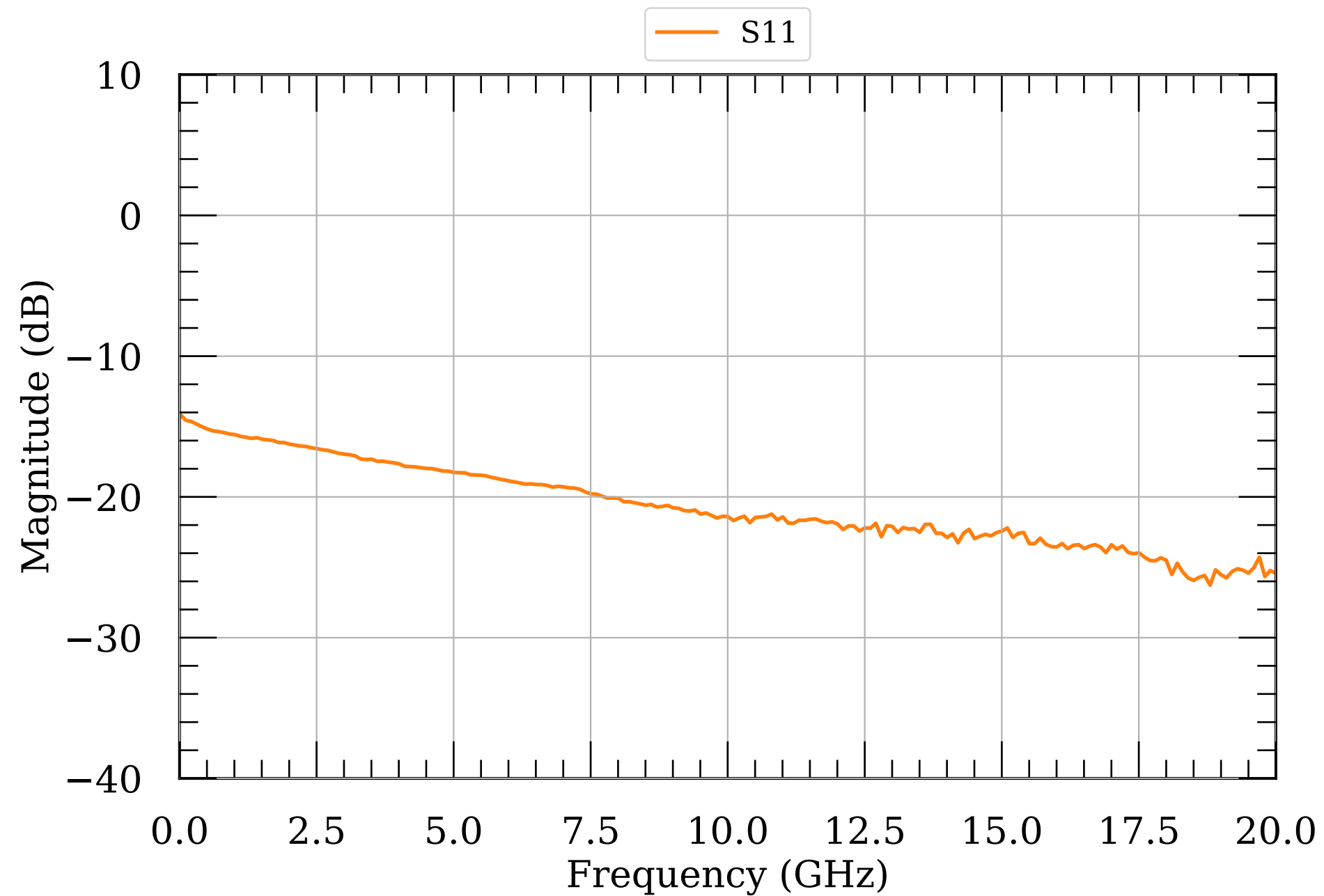
LNA S-params 6.5
