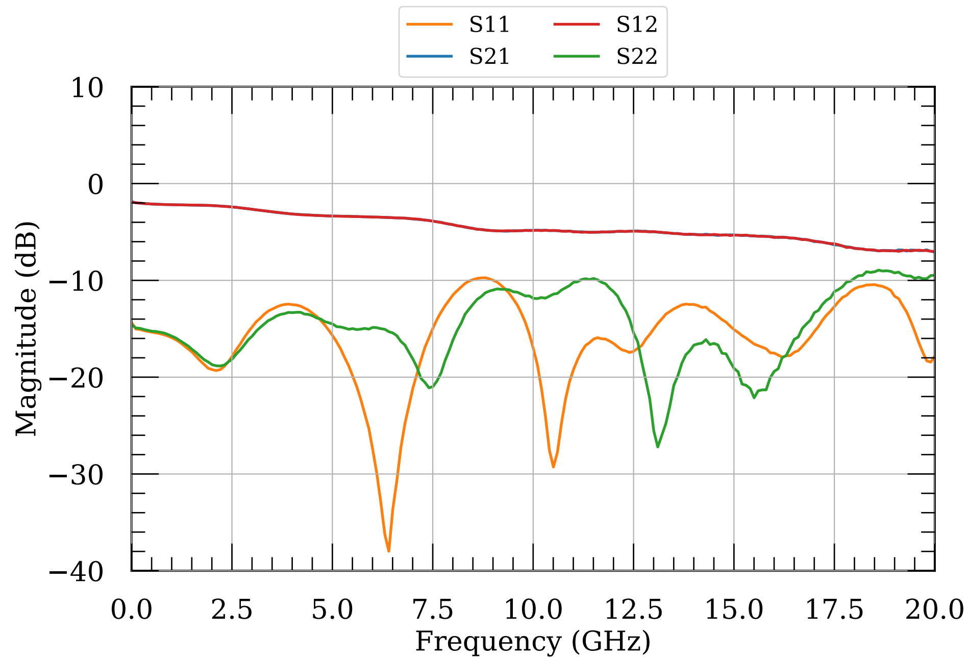
LNA S-params, 0 dBm
