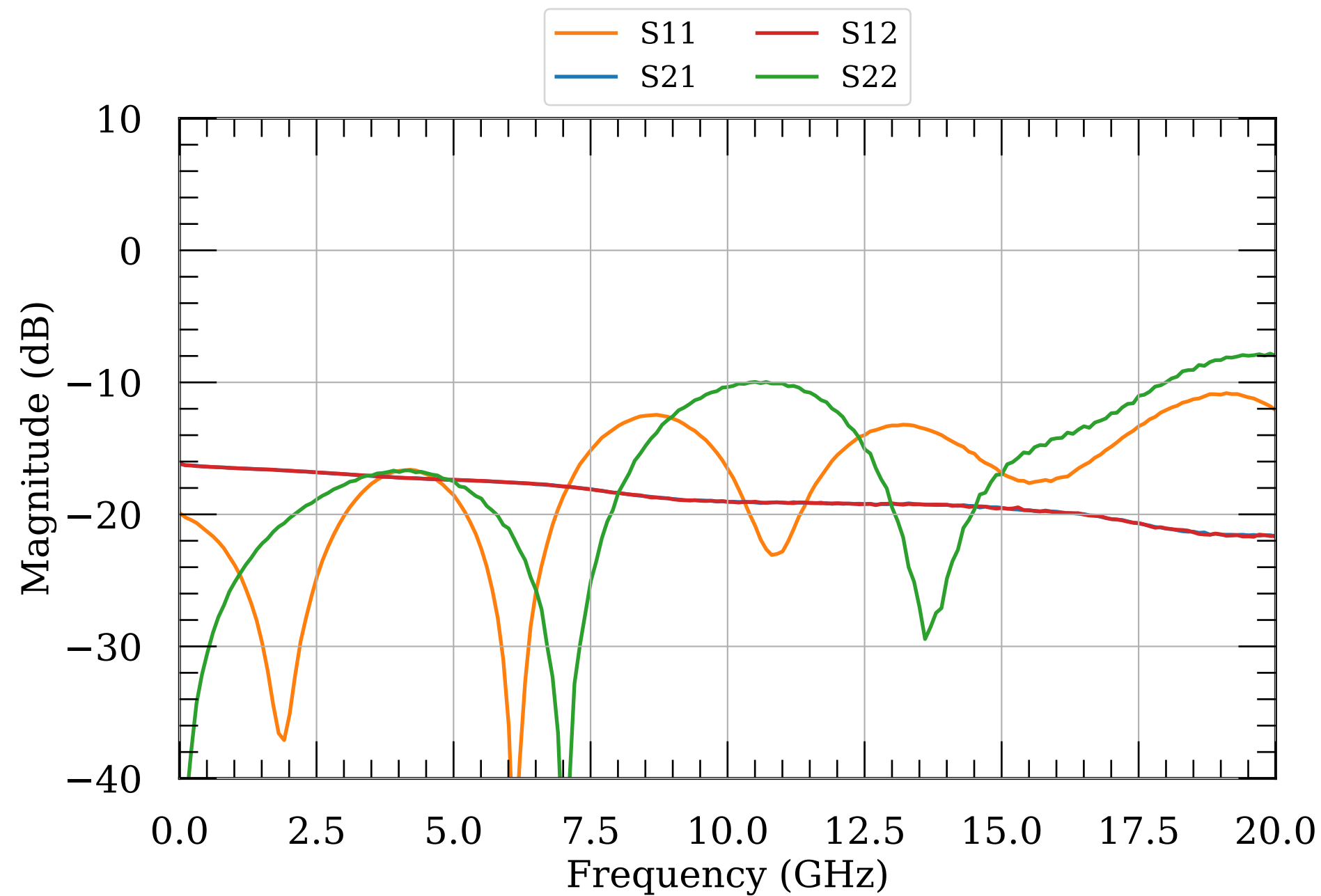
LNA S-params, 14 dBm
