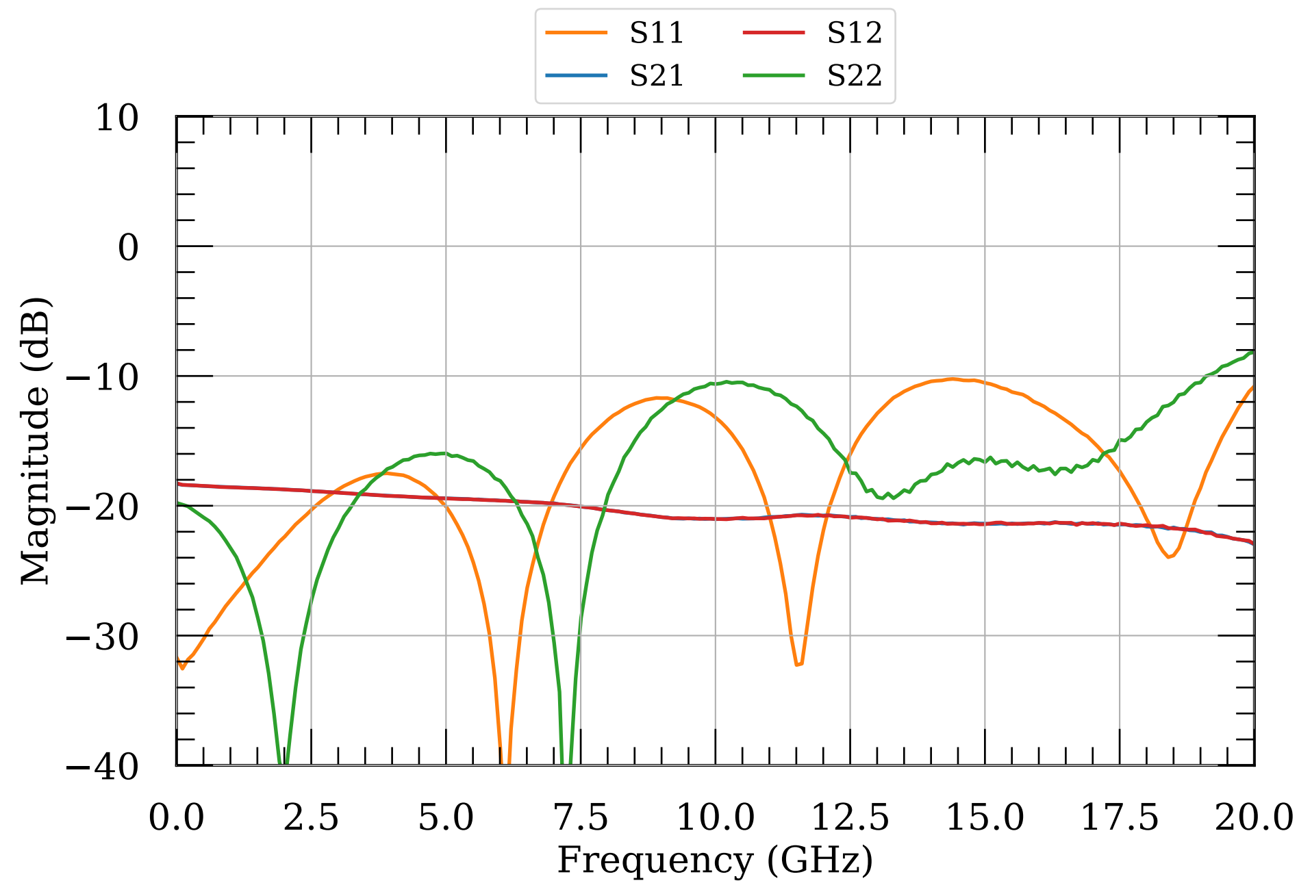
LNA S-params, 16 dBm
