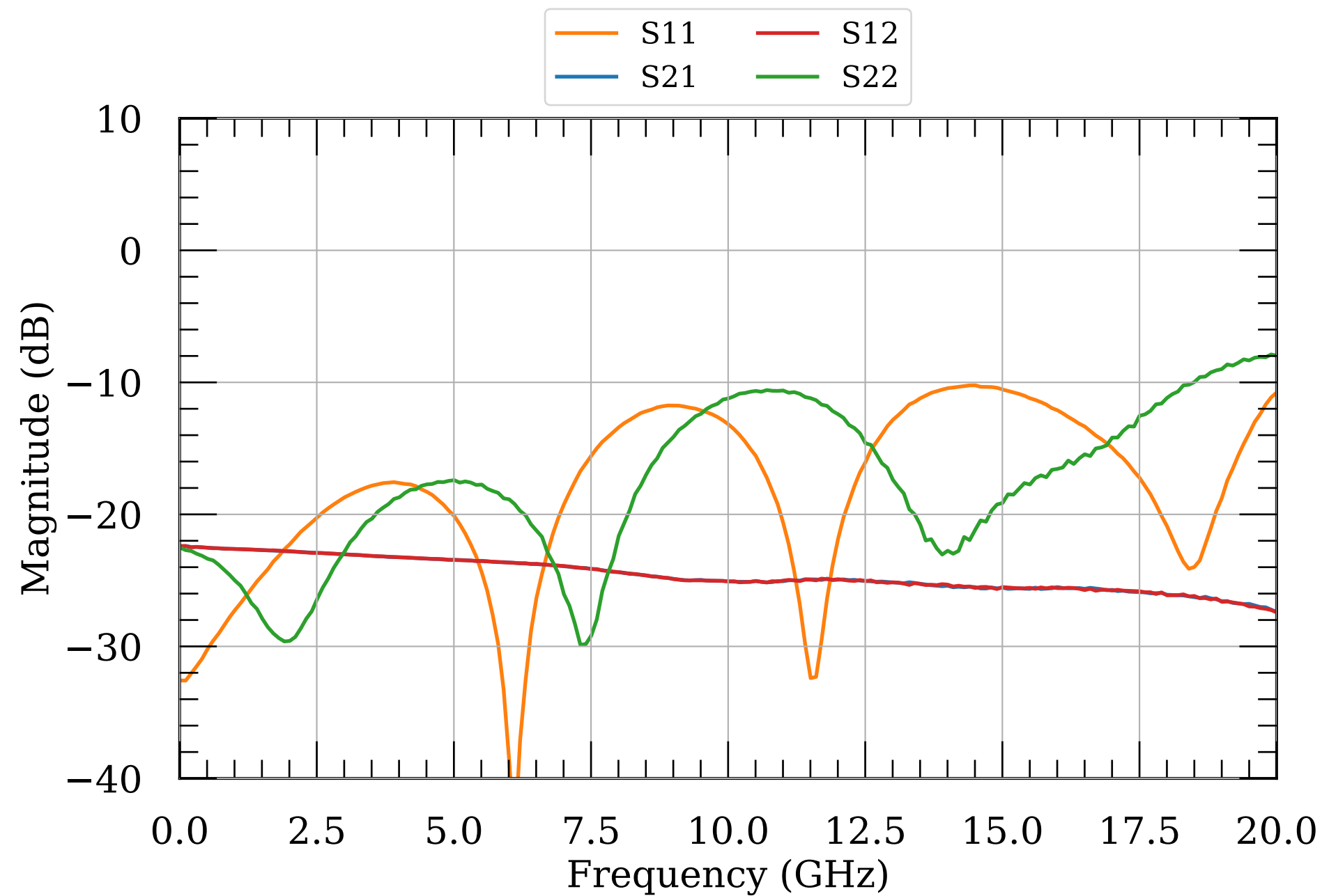
LNA S-params, 20 dBm
