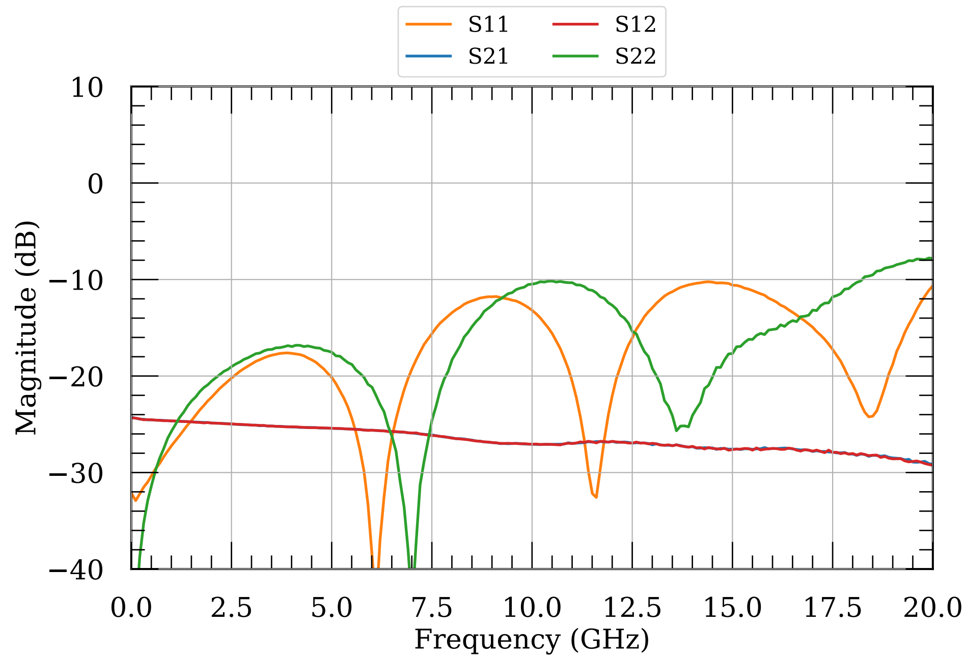
LNA S-params, 22 dBm
