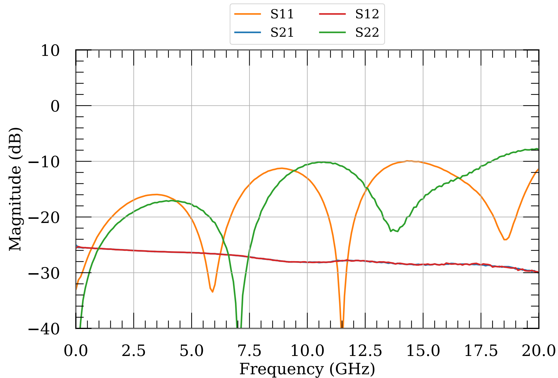
LNA S-params, 23 dBm
