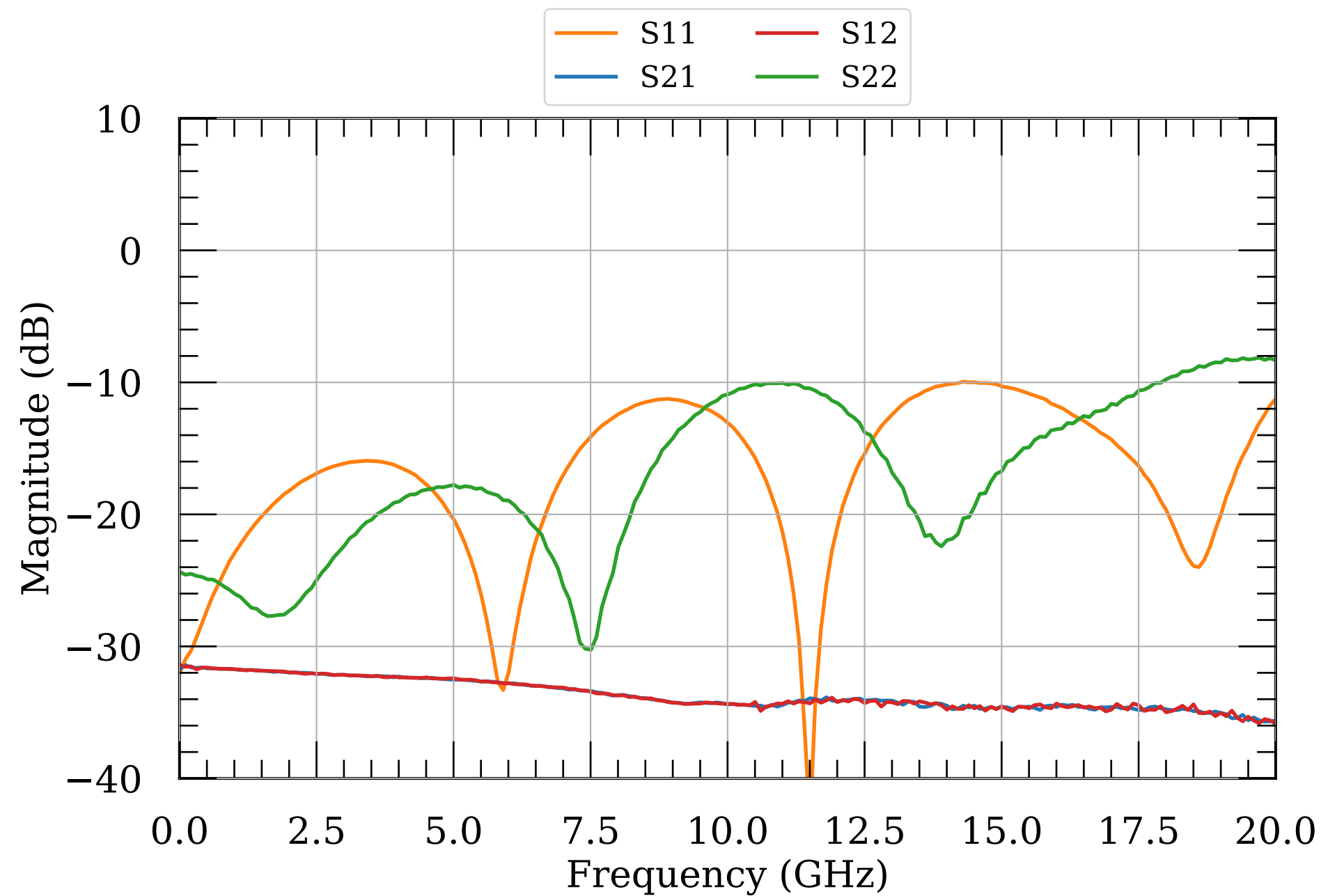
LNA S-params, 29 dBm
