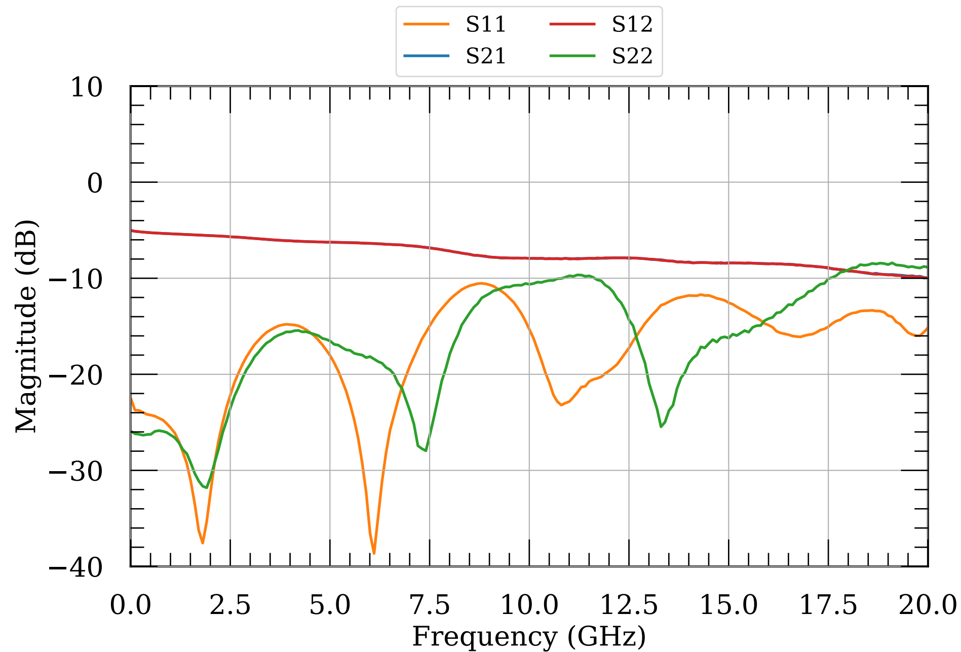
LNA S-params, 3 dBm
