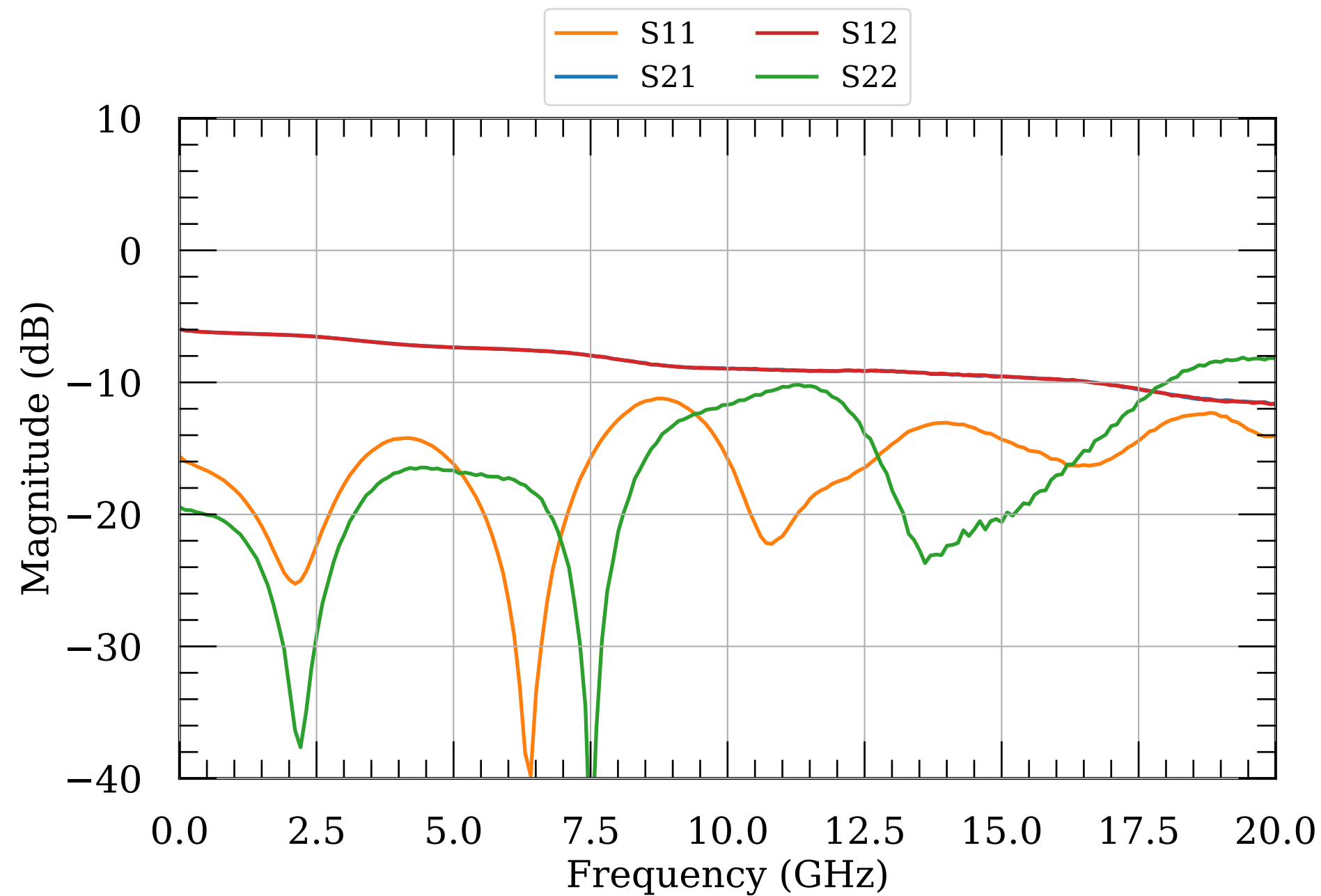
LNA S-params, 4 dBm
