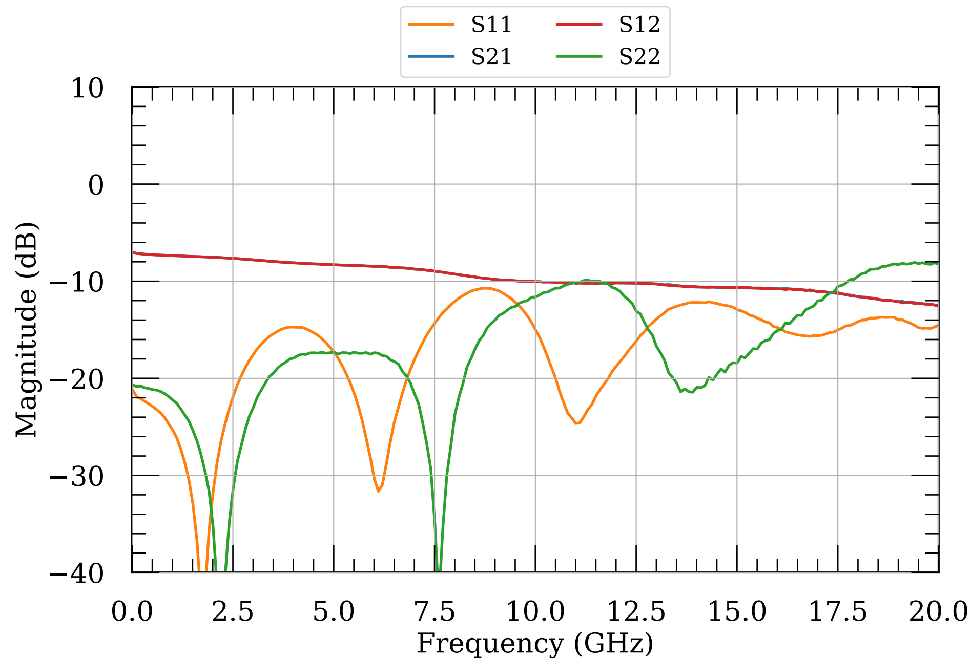
LNA S-params, 5 dBm
