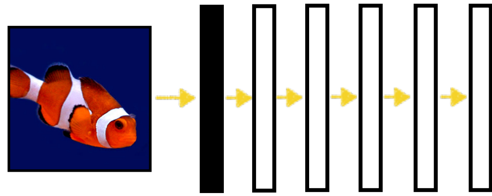
Layer 1 representation
