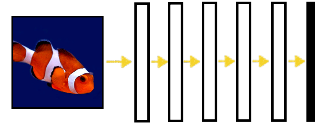
Layer 6 representation
