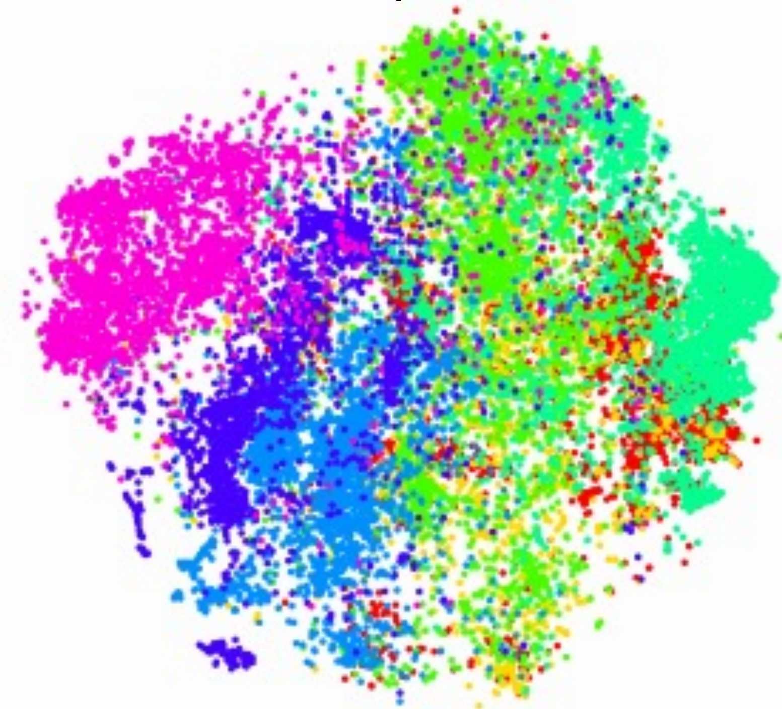
Layer 6 representation
