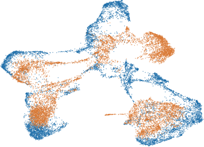
STEP graph-aggregated
