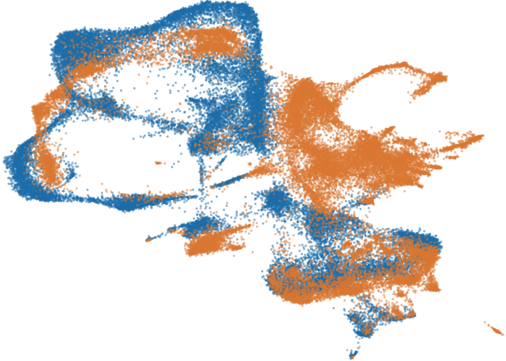
NicheCompass latent
