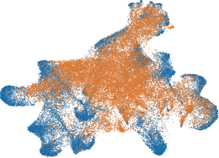
STEP no-graph
