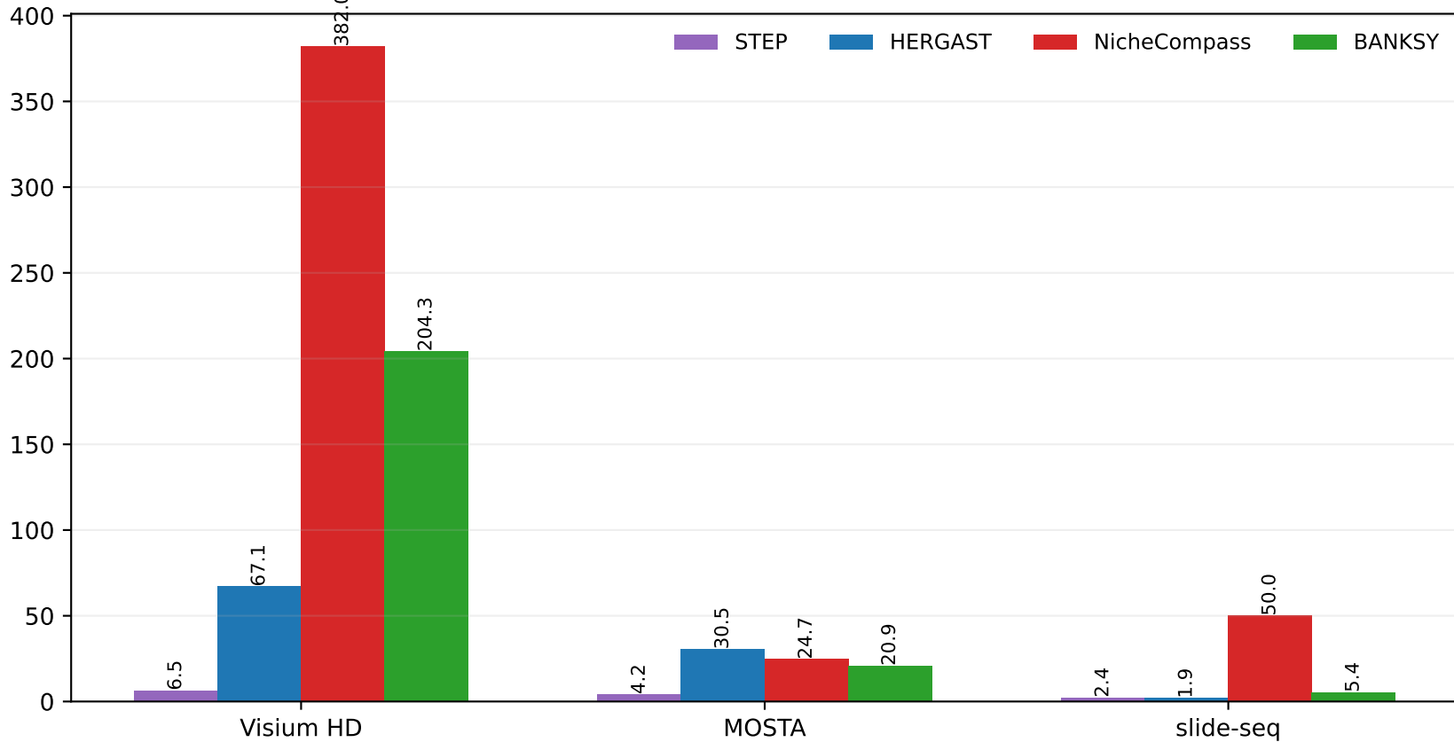
Runtime
