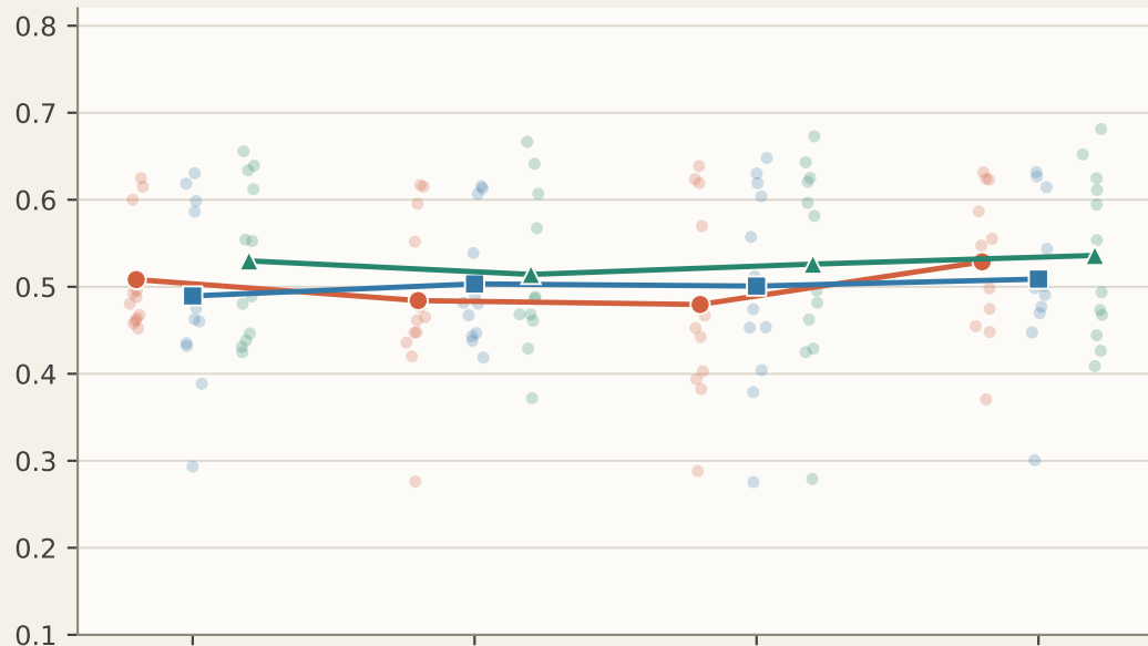
GraphST ARI
