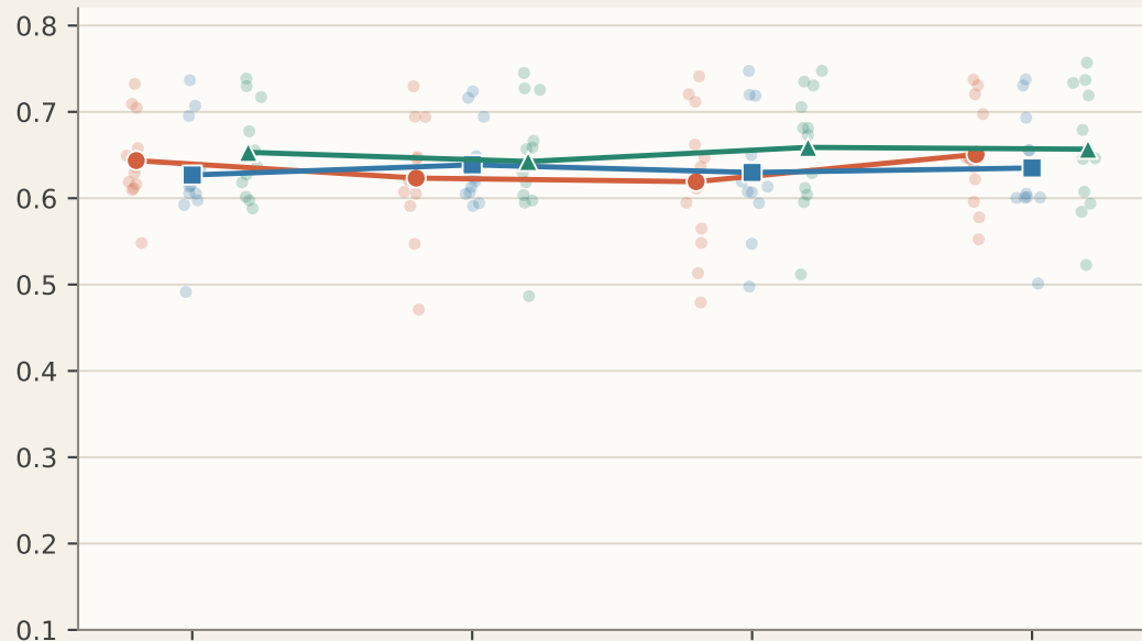
GraphST NMI
