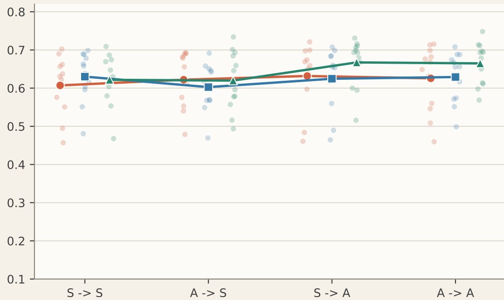
STAGATE NMI
