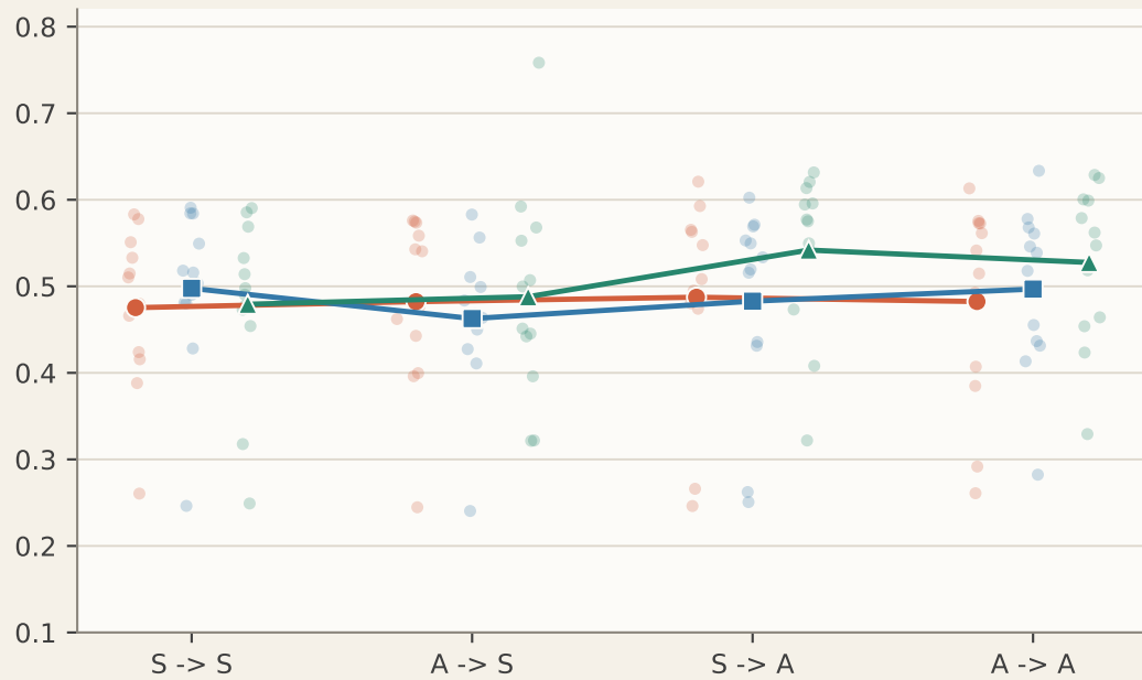
STAGATE ARI
