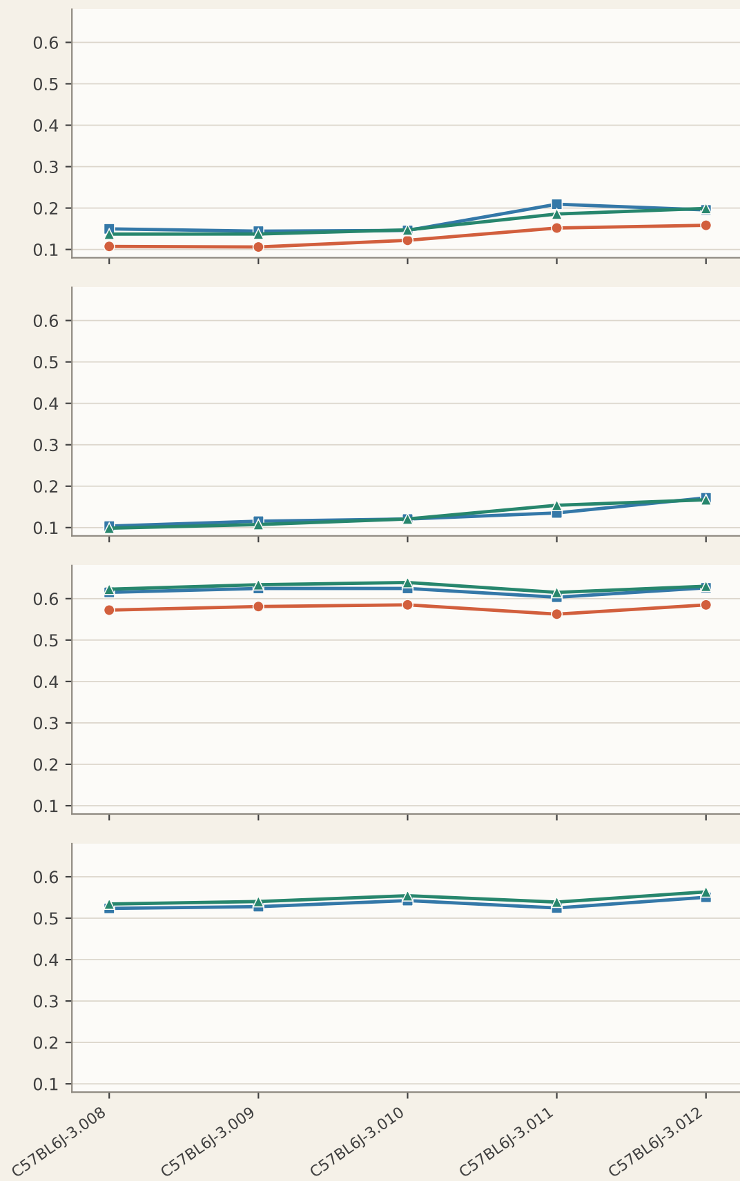
CCF regions
