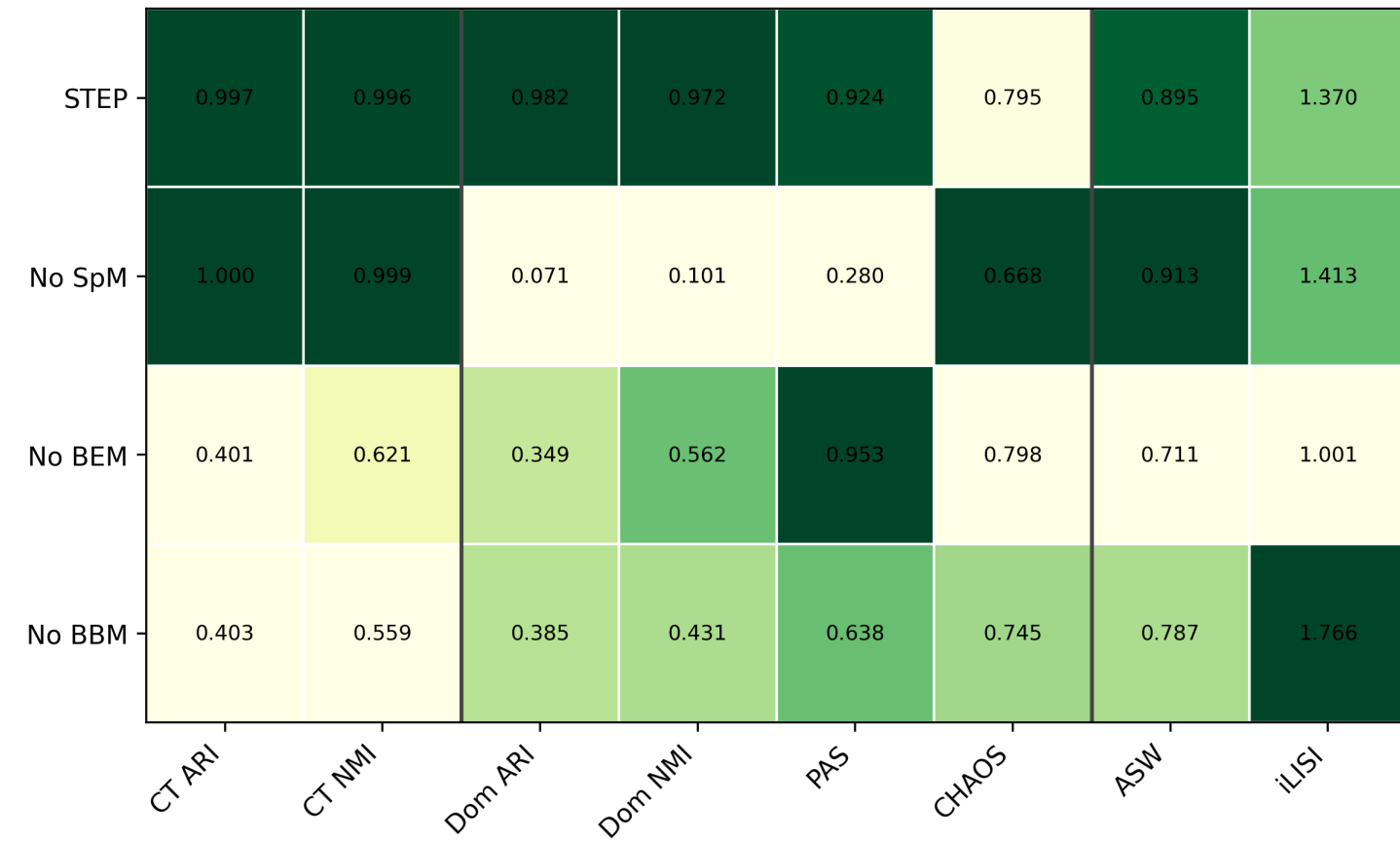
Batch effect
