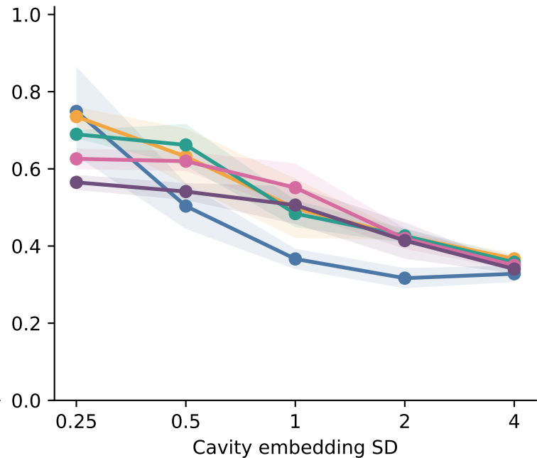
ARI
