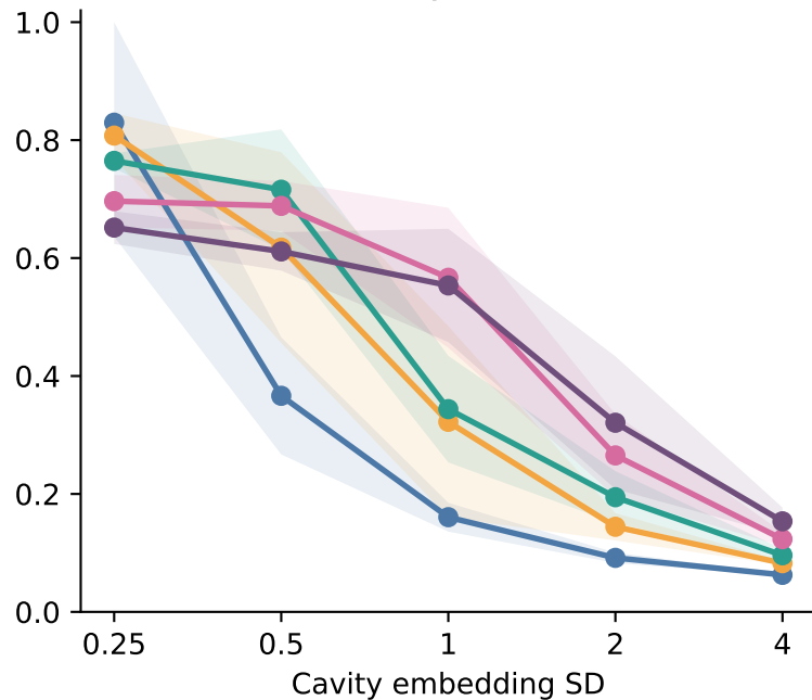
Cavity recall
