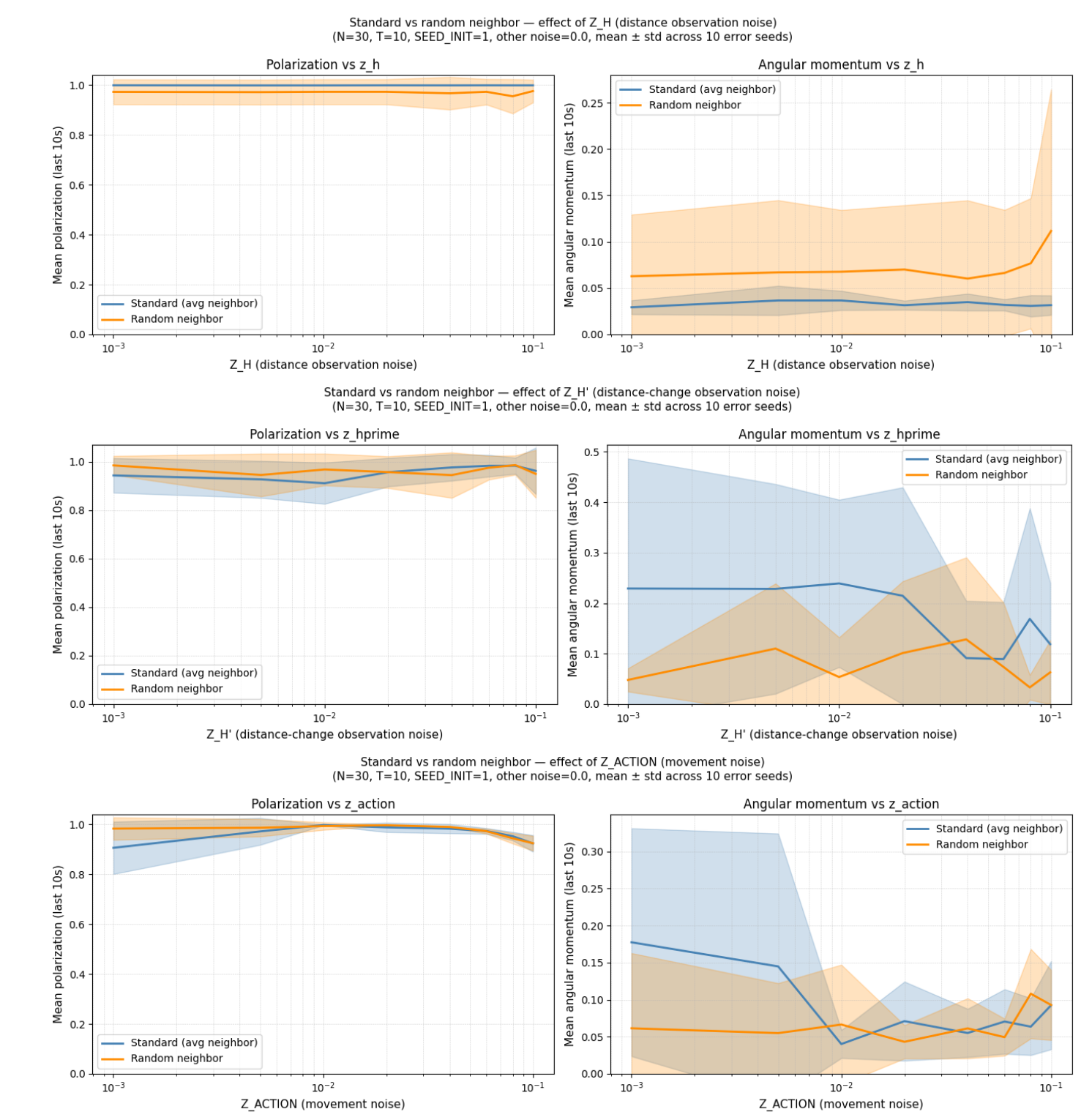
Figure 3. The average polarization and angular momentum values across ten noise realization seeds at different Z values for the average and random neighbor branches (from the top down: Z_H , Z_{H'} , and Z_{Action} ). The shaded portions of the graphs represent a \pm 1 standard deviation region.
