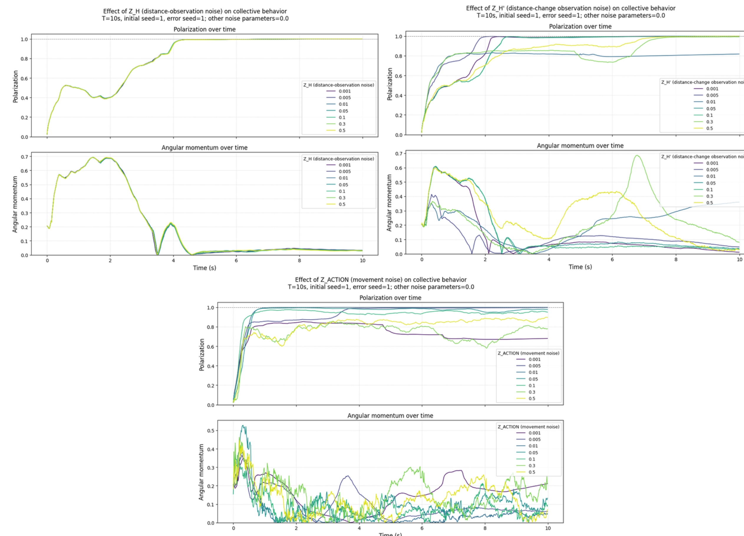
Figure 2. The group polarization and angular momentum across different Z noise parameter values [clockwise from top left: Z_H , Z_{H'} , and Z_{Action} ]. Plotted runs lasted 10 seconds and only one noise parameter type was active per run.
