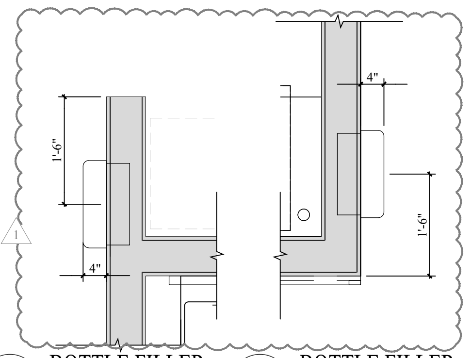
04 BOTTLE FILLER 3/4" = 1'-0" 03 BOTTLE FILLER 3/4" = 1'-0"
