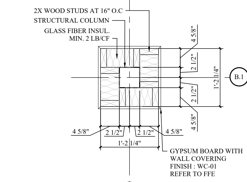
02 COLUMN DETAIL 1" = 1'-0"
