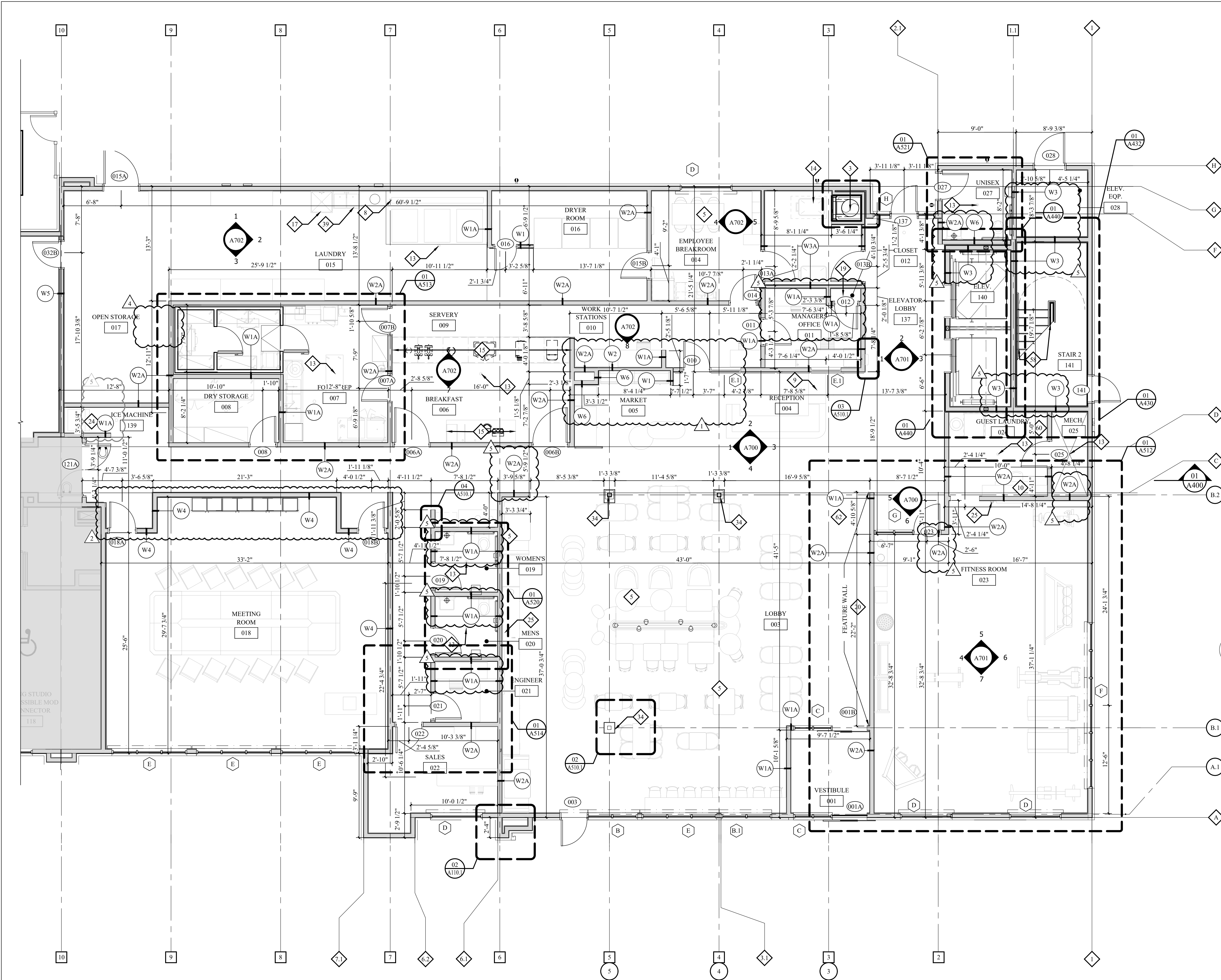
01 LOBBY AREA - CONSTRUCTION PLAN 3/16" = 1'-0"
